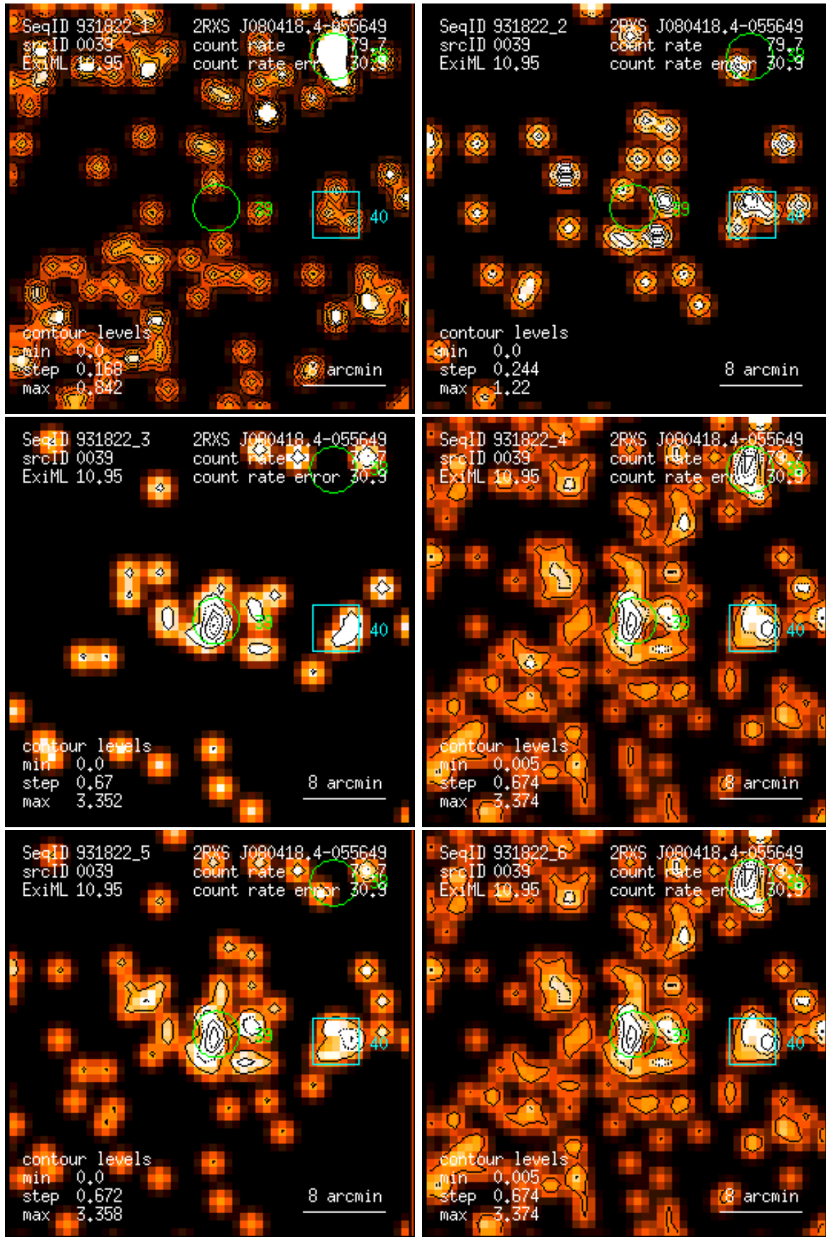
Figure 39: RASS 931822: detection 0039: band rate images, Gaussian filter: (1) PSPC channels 11 – 41, (2) 52 – 90, (3) 91 – 201, (4) 11 – 235, (5) 52 – 201, (6) 11 – 201. Broad band rates in counts/ks. Band rate contour levels in counts/ks/arcmin 2 .
