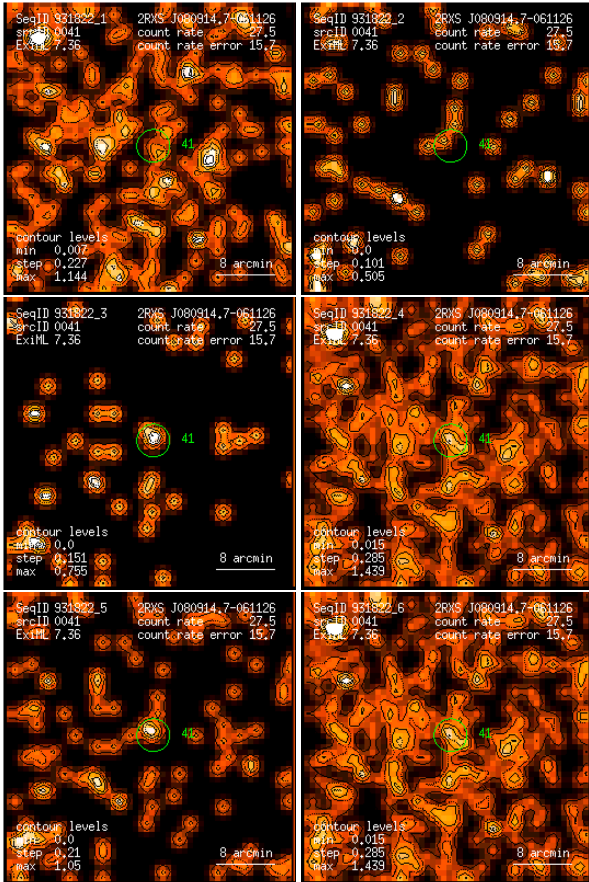
Figure 41: RASS 931822: detection 0041: band rate images, Gaussian filter: (1) PSPC channels 11 – 41, (2) 52 – 90, (3) 91 – 201, (4) 11 – 235, (5) 52 – 201, (6) 11 – 201. Broad band rates in counts/ks. Band rate contour levels in counts/ks/arcmin 2 .
