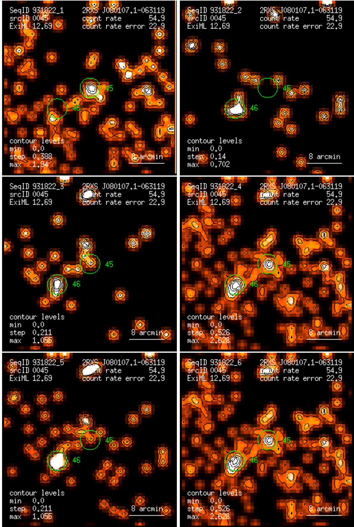
Figure 45: RASS 931822: detection 0045: band rate images, Gaussian filter: (1) PSPC channels 11 – 41, (2) 52 – 90, (3) 91 – 201, (4) 11 – 235, (5) 52 – 201, (6) 11 – 201. Broad band rates in counts/ks. Band rate contour levels in counts/ks/arcmin 2 .
