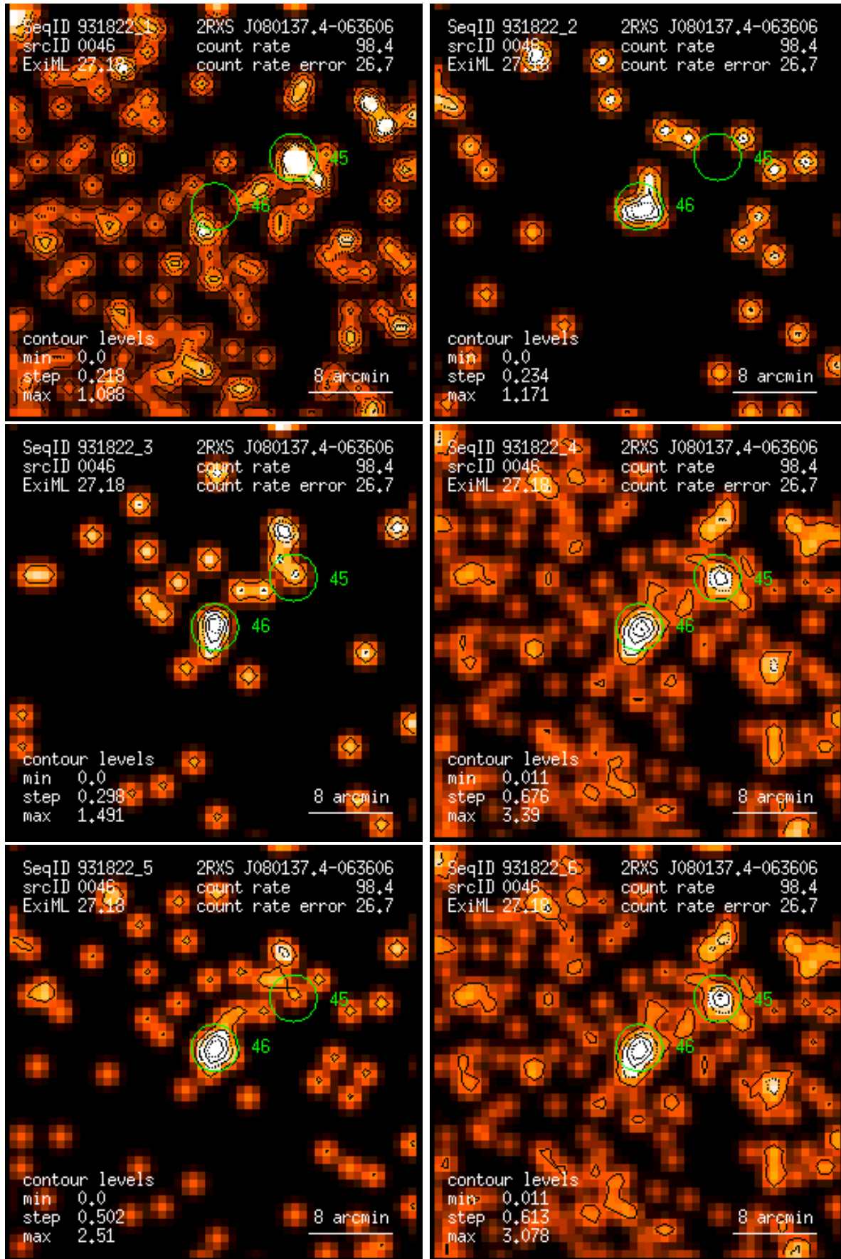
Figure 46: RASS 931822: detection 0046: band rate images, Gaussian filter: (1) PSPC channels 11 – 41, (2) 52 – 90, (3) 91 – 201, (4) 11 – 235, (5) 52 – 201, (6) 11 – 201. Broad band rates in counts/ks. Band rate contour levels in counts/ks/arcmin 2 .
