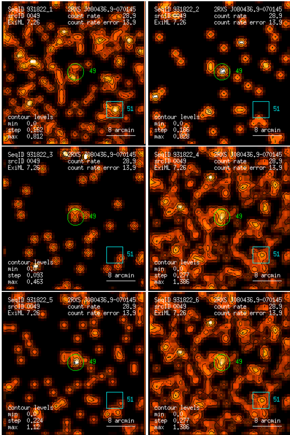
Figure 49: RASS 931822: detection 0049: band rate images, Gaussian filter: (1) PSPC channels 11 – 41, (2) 52 – 90, (3) 91 – 201, (4) 11 – 235, (5) 52 – 201, (6) 11 – 201. Broad band rates in counts/ks. Band rate contour levels in counts/ks/arcmin 2 .
