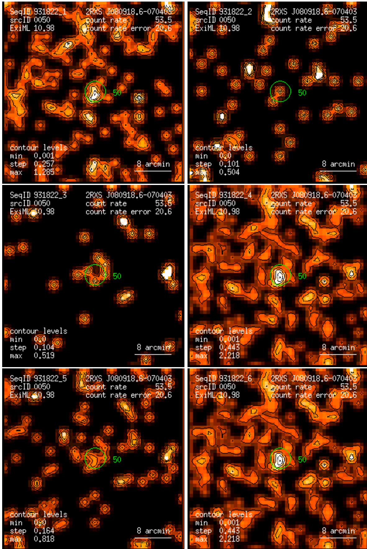
Figure 50: RASS 931822: detection 0050: band rate images, Gaussian filter: (1) PSPC channels 11 – 41, (2) 52 – 90, (3) 91 – 201, (4) 11 – 235, (5) 52 – 201, (6) 11 – 201. Broad band rates in counts/ks. Band rate contour levels in counts/ks/arcmin 2 .
