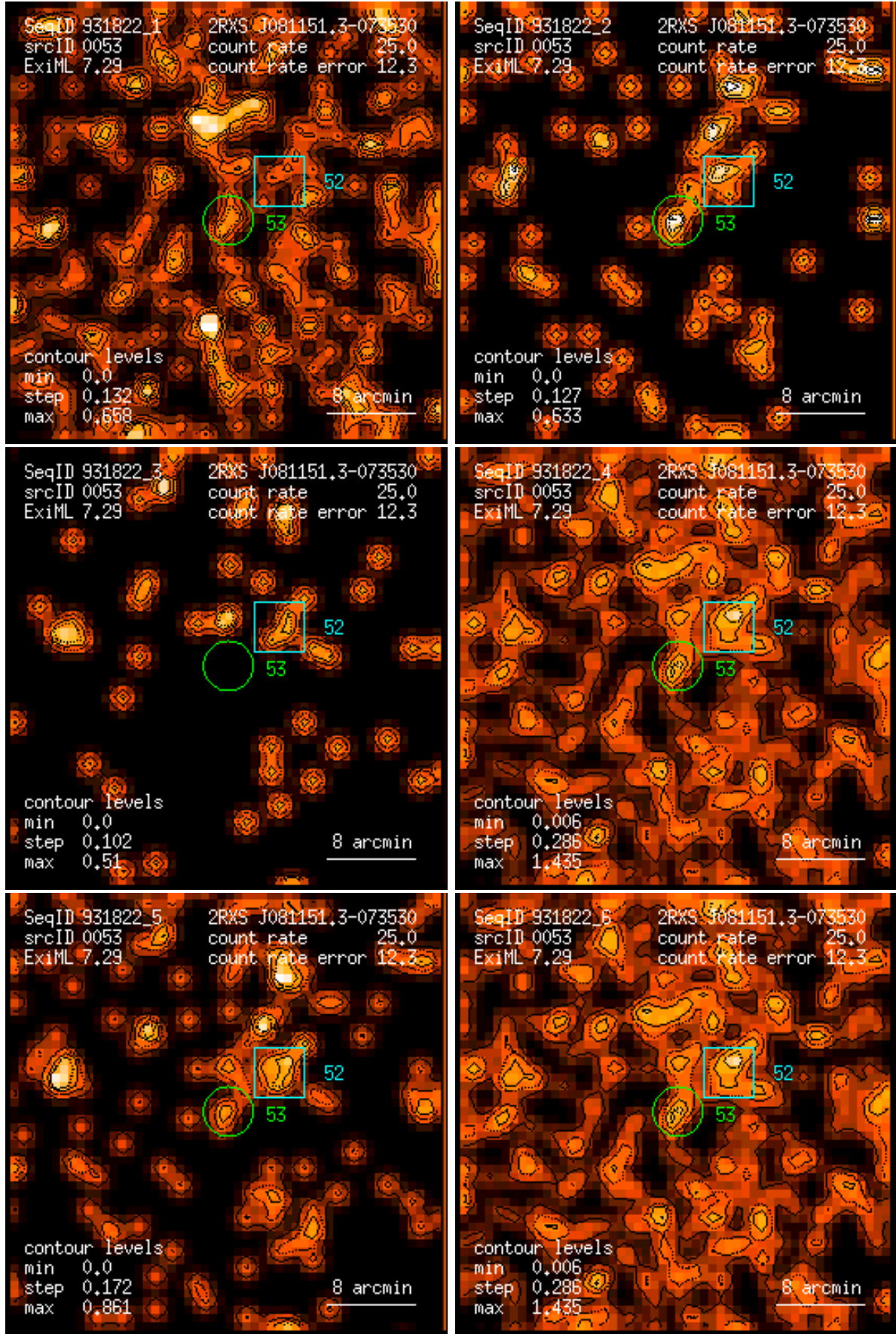
Figure 53: RASS 931822: detection 0053: band rate images, Gaussian filter: (1) PSPC channels 11 – 41, (2) 52 – 90, (3) 91 – 201, (4) 11 – 235, (5) 52 – 201, (6) 11 – 201. Broad band rates in counts/ks. Band rate contour levels in counts/ks/arcmin 2 .
