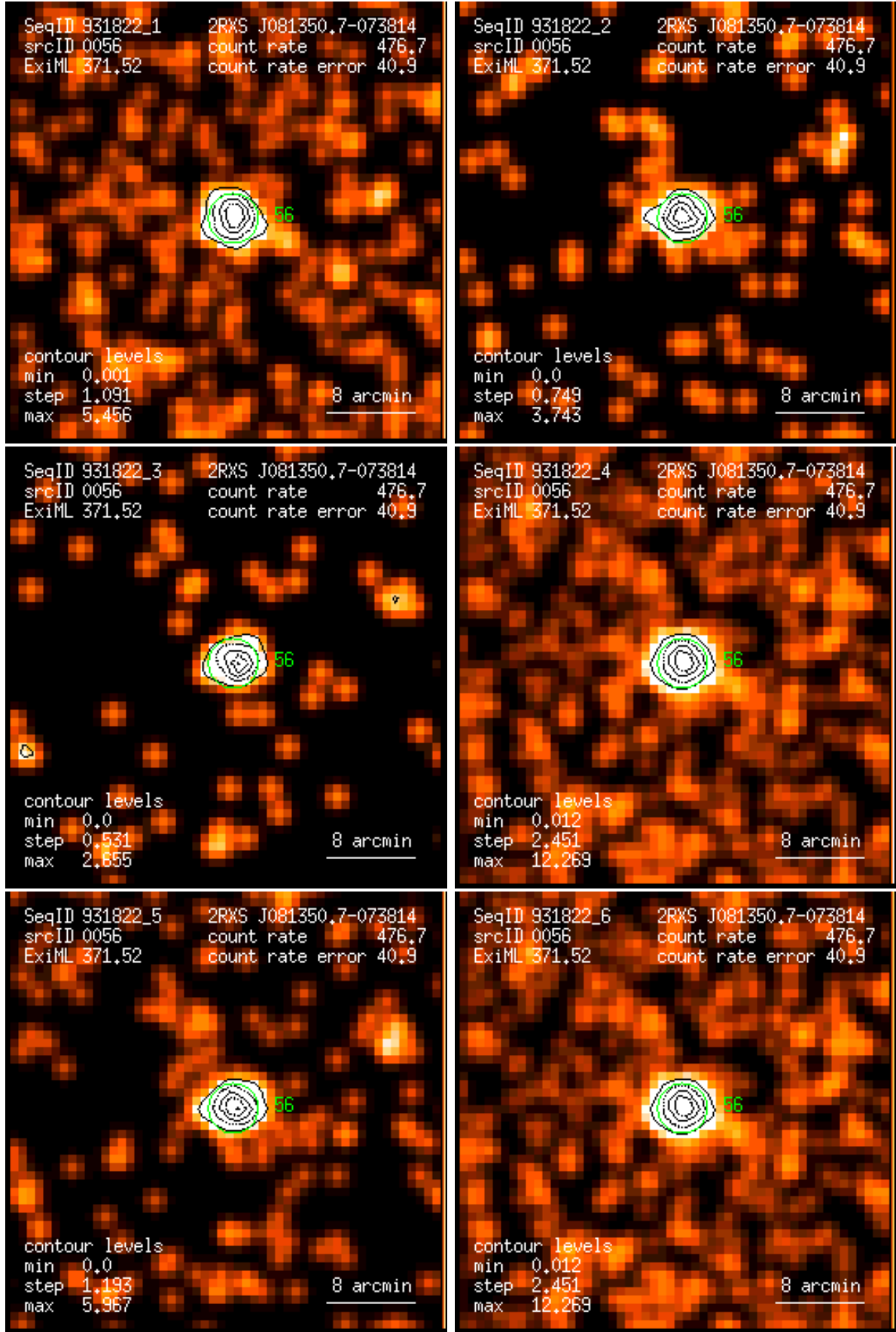
Figure 56: RASS 931822: detection 0056: band rate images, Gaussian filter: (1) PSPC channels 11 – 41, (2) 52 – 90, (3) 91 – 201, (4) 11 – 235, (5) 52 – 201, (6) 11 – 201. Broad band rates in counts/ks. Band rate contour levels in counts/ks/arcmin 2 .
