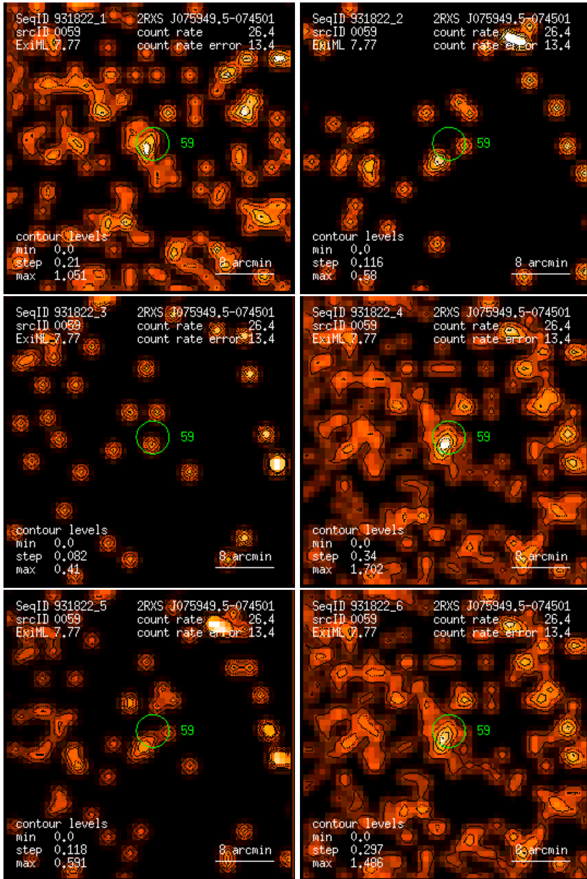
Figure 59: RASS 931822: detection 0059: band rate images, Gaussian filter: (1) PSPC channels 11 – 41, (2) 52 – 90, (3) 91 – 201, (4) 11 – 235, (5) 52 – 201, (6) 11 – 201. Broad band rates in counts/ks. Band rate contour levels in counts/ks/arcmin 2 .
