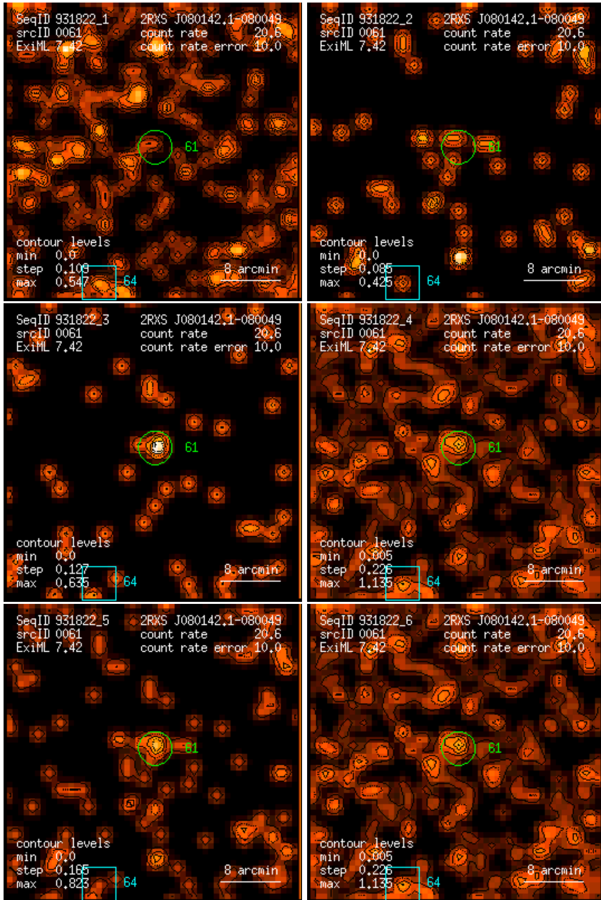
Figure 61: RASS 931822: detection 0061: band rate images, Gaussian filter: (1) PSPC channels 11 – 41, (2) 52 – 90, (3) 91 – 201, (4) 11 – 235, (5) 52 – 201, (6) 11 – 201. Broad band rates in counts/ks. Band rate contour levels in counts/ks/arcmin 2 .
