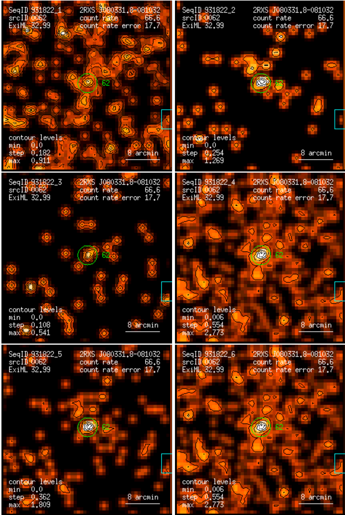
Figure 62: RASS 931822: detection 0062: band rate images, Gaussian filter: (1) PSPC channels 11 – 41, (2) 52 – 90, (3) 91 – 201, (4) 11 – 235, (5) 52 – 201, (6) 11 – 201. Broad band rates in counts/ks. Band rate contour levels in counts/ks/arcmin 2 .
