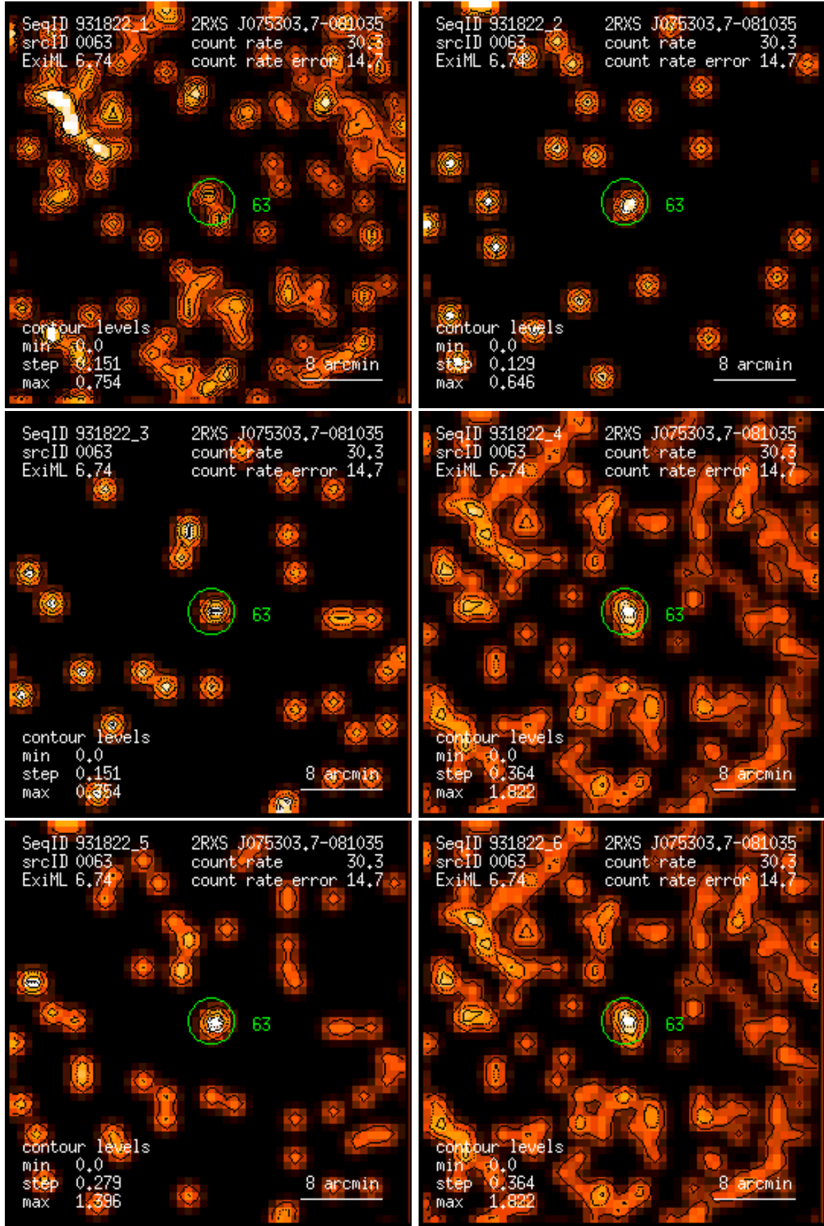
Figure 63: RASS 931822: detection 0063: band rate images, Gaussian filter: (1) PSPC channels 11 – 41, (2) 52 – 90, (3) 91 – 201, (4) 11 – 235, (5) 52 – 201, (6) 11 – 201. Broad band rates in counts/ks. Band rate contour levels in counts/ks/arcmin 2 .
