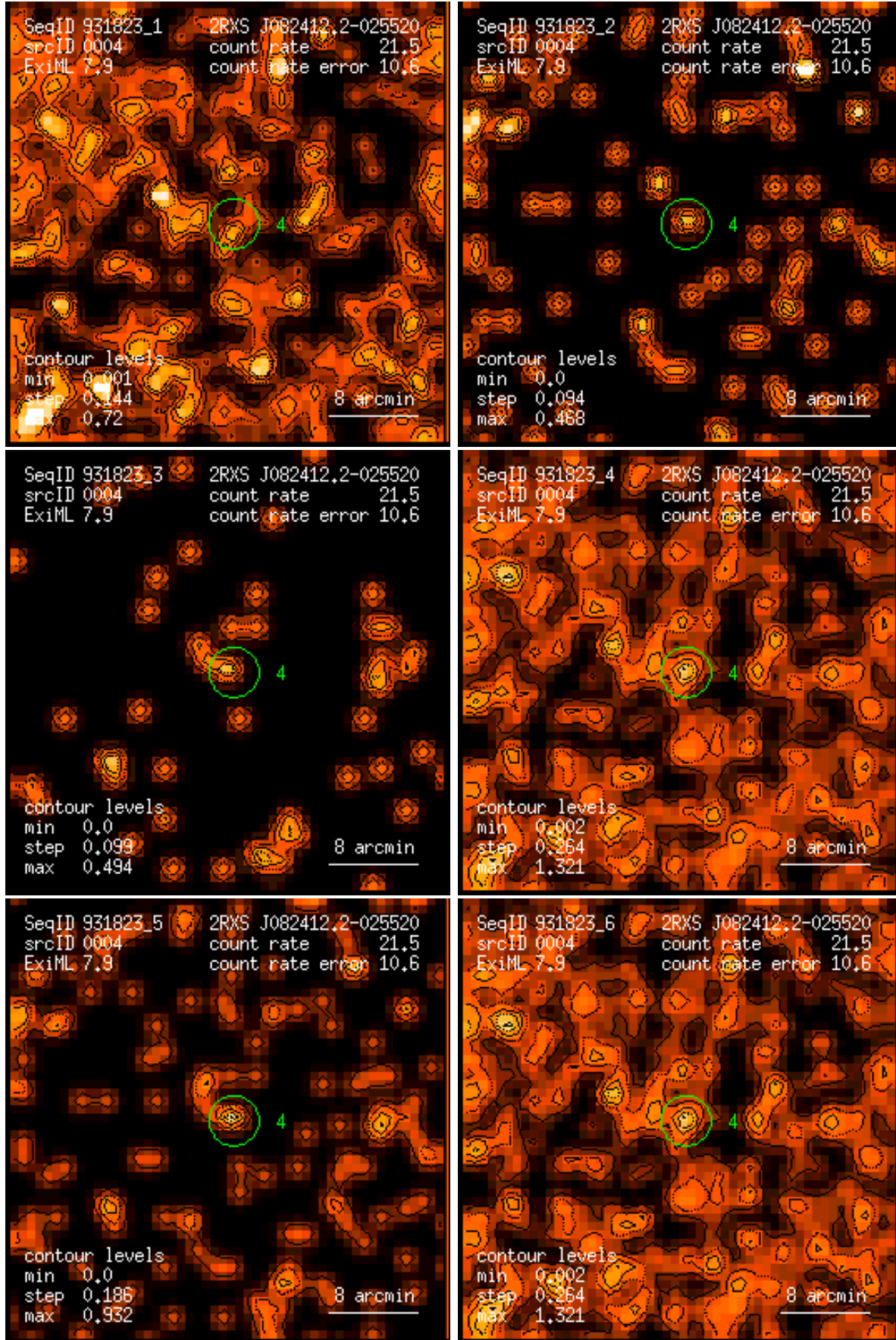
Figure 4: RASS 931823: detection 0004: band rate images, Gaussian filter: (1) PSPC channels 11 – 41, (2) 52 – 90, (3) 91 – 201, (4) 11 – 235, (5) 52 – 201, (6) 11 – 201. Broad band rates in counts/ks. Band rate contour levels in counts/ks/arcmin 2 .
