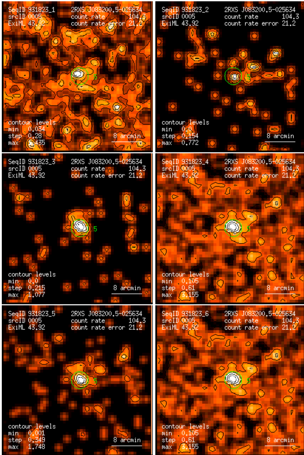
Figure 5: RASS 931823: detection 0005: band rate images, Gaussian filter: (1) PSPC channels 11 – 41, (2) 52 – 90, (3) 91 – 201, (4) 11 – 235, (5) 52 – 201, (6) 11 – 201. Broad band rates in counts/ks. Band rate contour levels in counts/ks/arcmin 2 .
