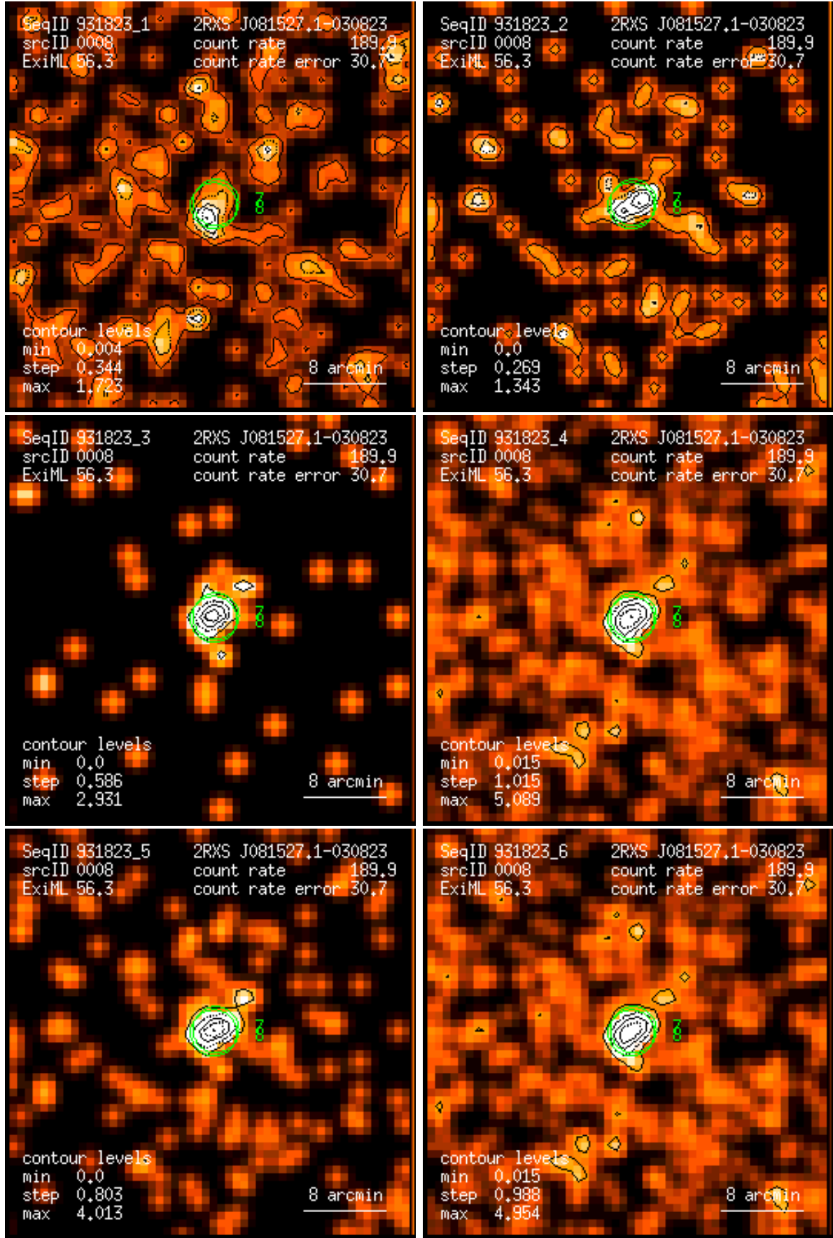
Figure 8: RASS 931823: detection 0008: band rate images, Gaussian filter: (1) PSPC channels 11 – 41, (2) 52 – 90, (3) 91 – 201, (4) 11 – 235, (5) 52 – 201, (6) 11 – 201. Broad band rates in counts/ks. Band rate contour levels in counts/ks/arcmin 2 .
