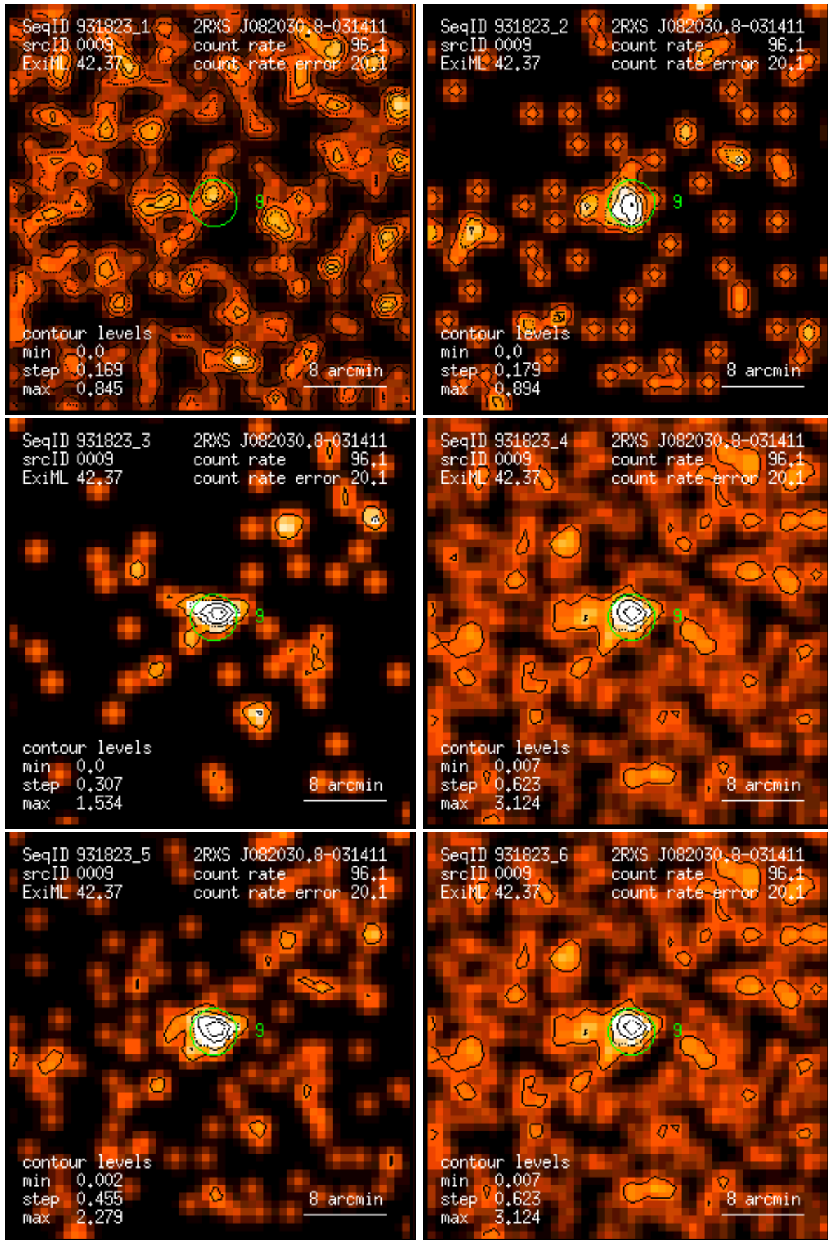
Figure 9: RASS 931823: detection 0009: band rate images, Gaussian filter: (1) PSPC channels 11 – 41, (2) 52 – 90, (3) 91 – 201, (4) 11 – 235, (5) 52 – 201, (6) 11 – 201. Broad band rates in counts/ks. Band rate contour levels in counts/ks/arcmin 2 .
