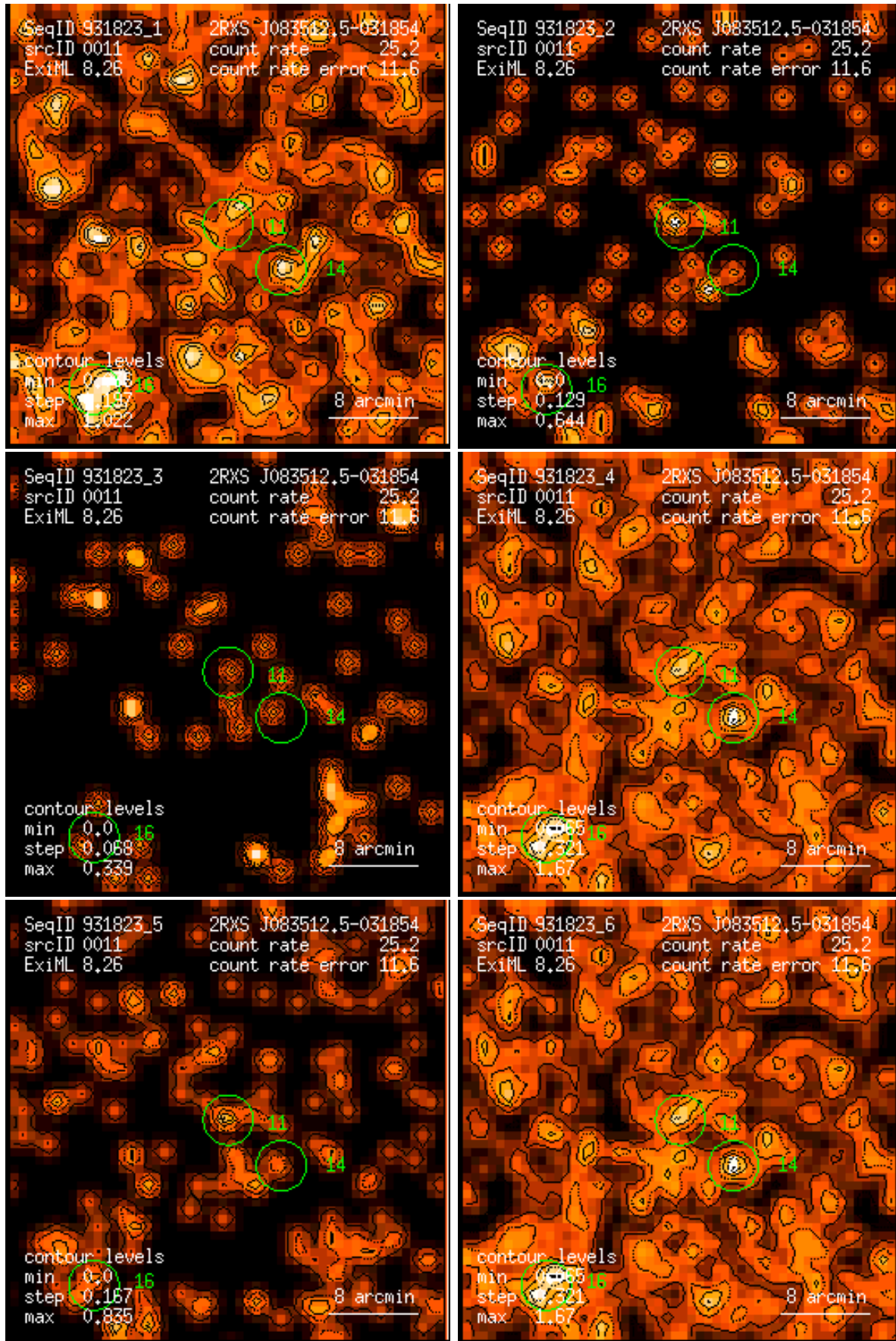
Figure 11: RASS 931823: detection 0011: band rate images, Gaussian filter: (1) PSPC channels 11 – 41, (2) 52 – 90, (3) 91 – 201, (4) 11 – 235, (5) 52 – 201, (6) 11 – 201. Broad band rates in counts/ks. Band rate contour levels in counts/ks/arcmin 2 .
