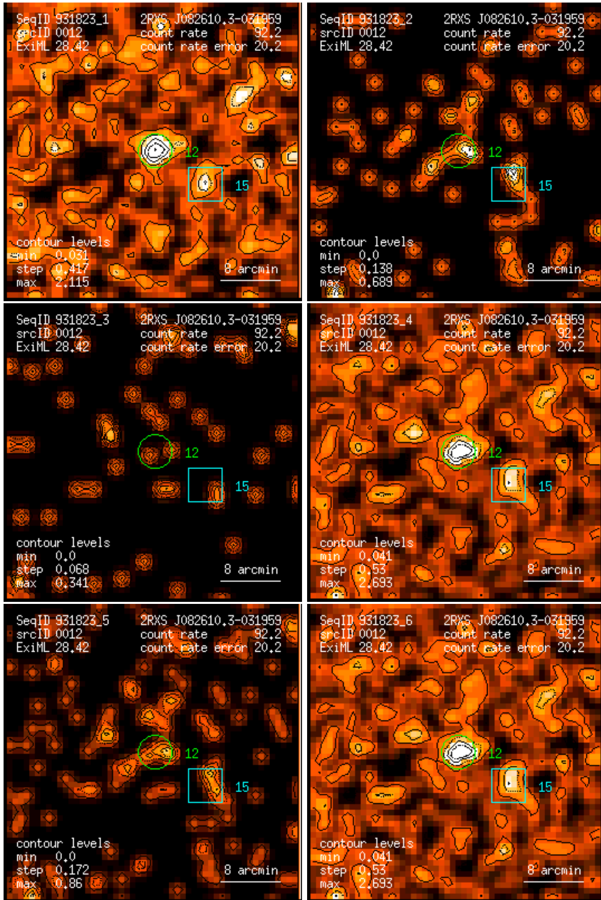
Figure 12: RASS 931823: detection 0012: band rate images, Gaussian filter: (1) PSPC channels 11 – 41, (2) 52 – 90, (3) 91 – 201, (4) 11 – 235, (5) 52 – 201, (6) 11 – 201. Broad band rates in counts/ks. Band rate contour levels in counts/ks/arcmin 2 .
