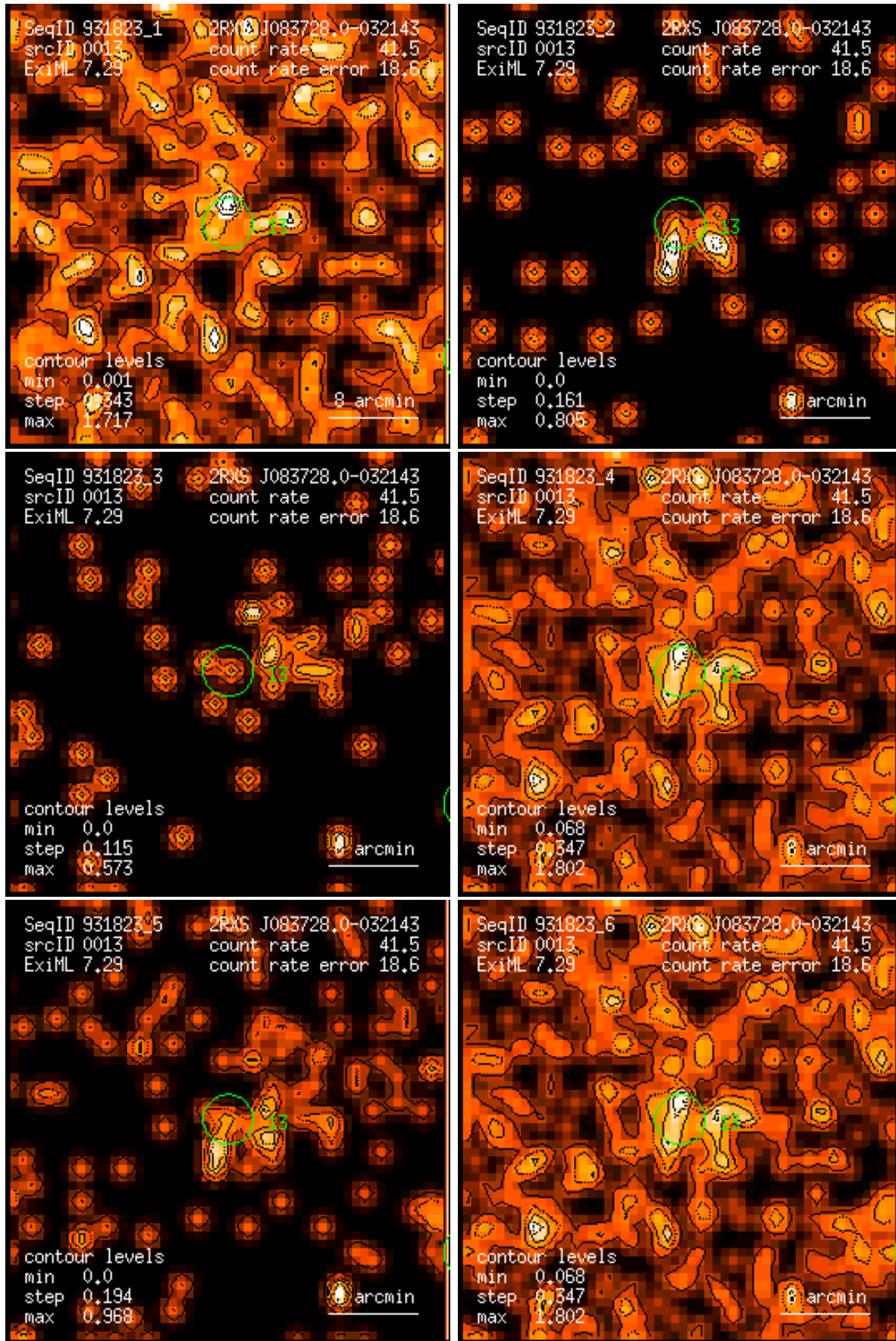
Figure 13: RASS 931823: detection 0013: band rate images, Gaussian filter: (1) PSPC channels 11 – 41, (2) 52 – 90, (3) 91 – 201, (4) 11 – 235, (5) 52 – 201, (6) 11 – 201. Broad band rates in counts/ks. Band rate contour levels in counts/ks/arcmin 2 .
