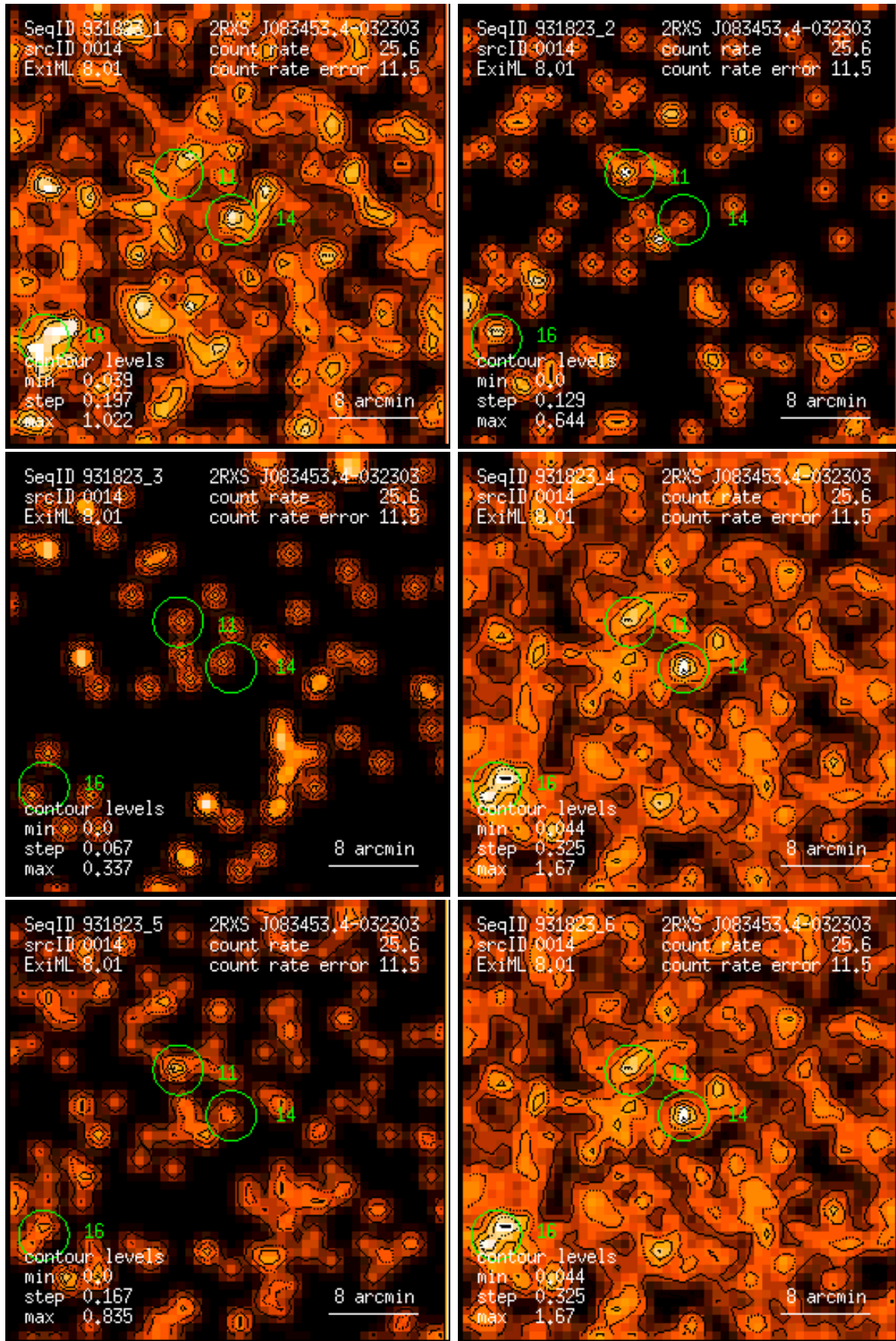
Figure 14: RASS 931823: detection 0014: band rate images, Gaussian filter: (1) PSPC channels 11 – 41, (2) 52 – 90, (3) 91 – 201, (4) 11 – 235, (5) 52 – 201, (6) 11 – 201. Broad band rates in counts/ks. Band rate contour levels in counts/ks/arcmin 2 .
