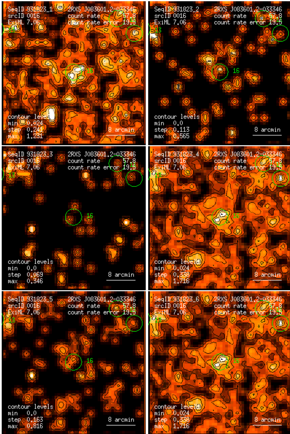
Figure 16: RASS 931823: detection 0016: band rate images, Gaussian filter: (1) PSPC channels 11 – 41, (2) 52 – 90, (3) 91 – 201, (4) 11 – 235, (5) 52 – 201, (6) 11 – 201. Broad band rates in counts/ks. Band rate contour levels in counts/ks/arcmin 2 .
