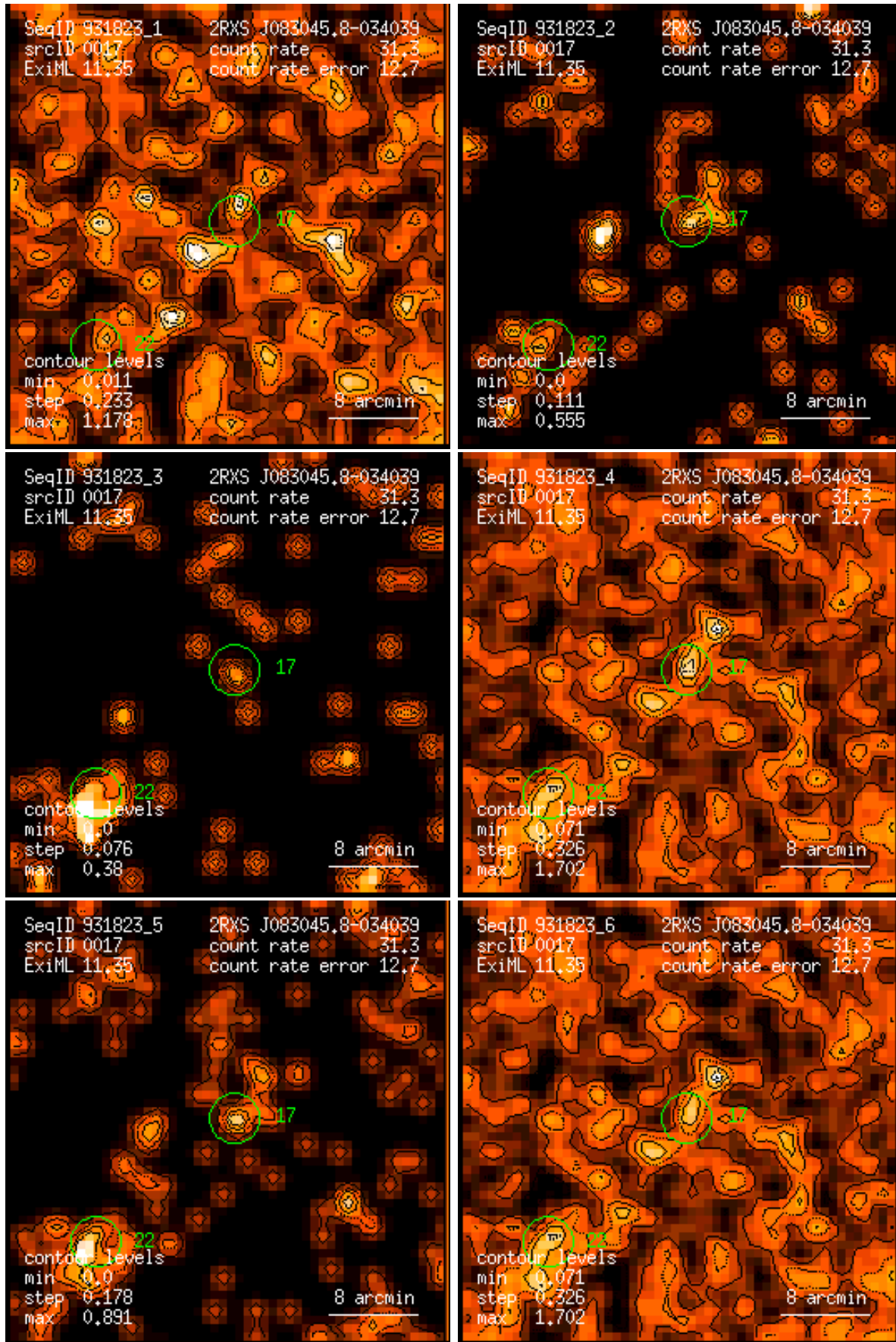
Figure 17: RASS 931823: detection 0017: band rate images, Gaussian filter: (1) PSPC channels 11 – 41, (2) 52 – 90, (3) 91 – 201, (4) 11 – 235, (5) 52 – 201, (6) 11 – 201. Broad band rates in counts/ks. Band rate contour levels in counts/ks/arcmin 2 .
