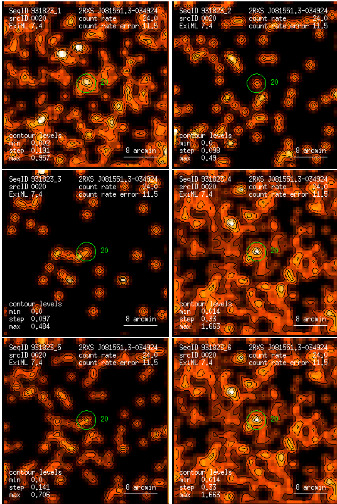
Figure 20: RASS 931823: detection 0020: band rate images, Gaussian filter: (1) PSPC channels 11 – 41, (2) 52 – 90, (3) 91 – 201, (4) 11 – 235, (5) 52 – 201, (6) 11 – 201. Broad band rates in counts/ks. Band rate contour levels in counts/ks/arcmin 2 .
