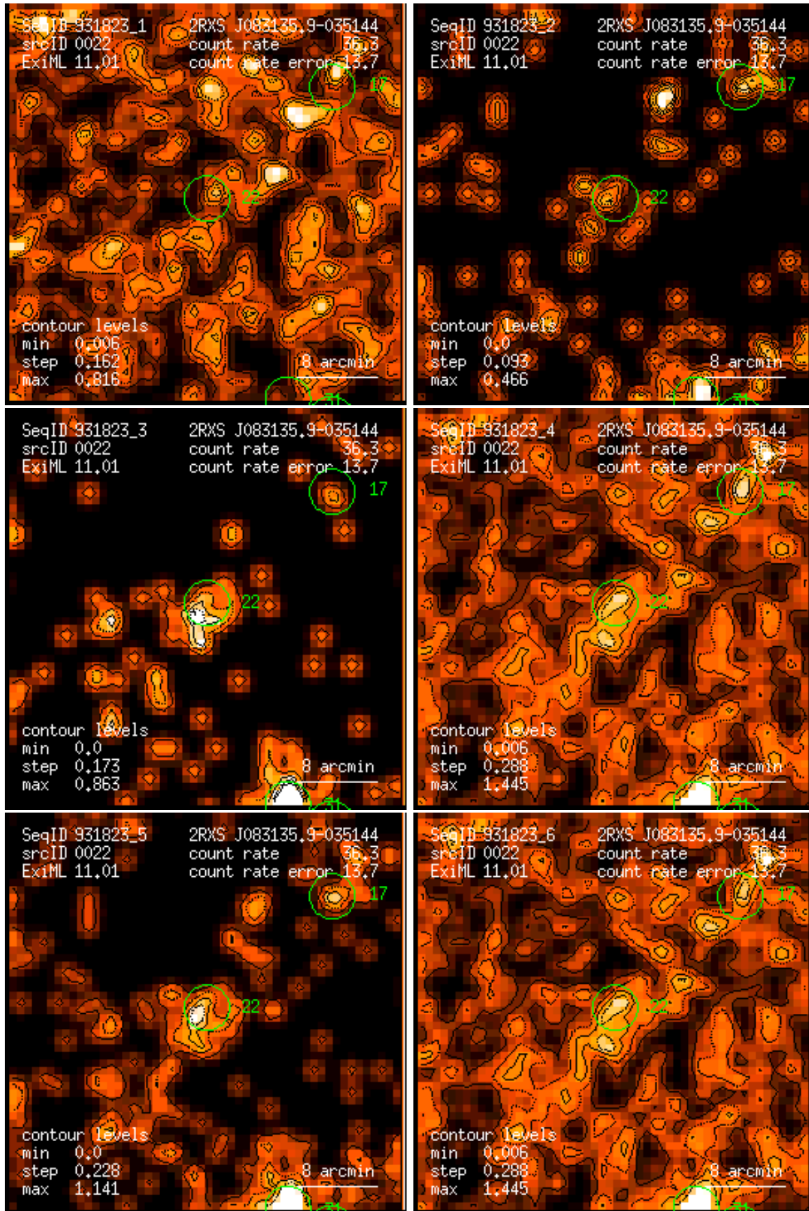
Figure 22: RASS 931823: detection 0022: band rate images, Gaussian filter: (1) PSPC channels 11 – 41, (2) 52 – 90, (3) 91 – 201, (4) 11 – 235, (5) 52 – 201, (6) 11 – 201. Broad band rates in counts/ks. Band rate contour levels in counts/ks/arcmin 2 .
