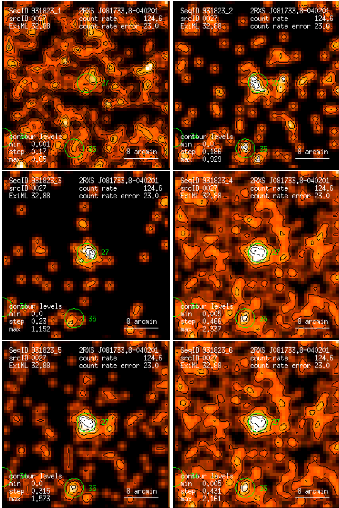
Figure 27: RASS 931823: detection 0027: band rate images, Gaussian filter: (1) PSPC channels 11 – 41, (2) 52 – 90, (3) 91 – 201, (4) 11 – 235, (5) 52 – 201, (6) 11 – 201. Broad band rates in counts/ks. Band rate contour levels in counts/ks/arcmin 2 .
