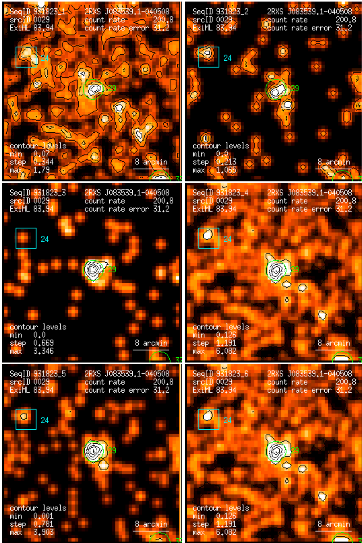
Figure 29: RASS 931823: detection 0029: band rate images, Gaussian filter: (1) PSPC channels 11 – 41, (2) 52 – 90, (3) 91 – 201, (4) 11 – 235, (5) 52 – 201, (6) 11 – 201. Broad band rates in counts/ks. Band rate contour levels in counts/ks/arcmin 2 .
