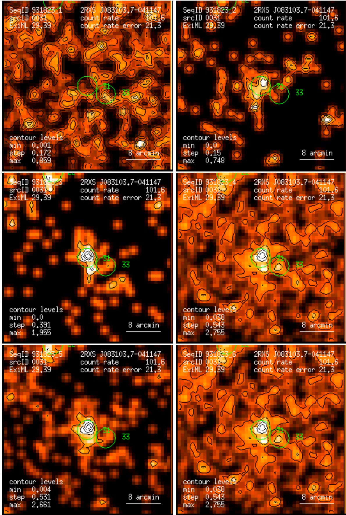
Figure 31: RASS 931823: detection 0031: band rate images, Gaussian filter: (1) PSPC channels 11 – 41, (2) 52 – 90, (3) 91 – 201, (4) 11 – 235, (5) 52 – 201, (6) 11 – 201. Broad band rates in counts/ks. Band rate contour levels in counts/ks/arcmin 2 .
