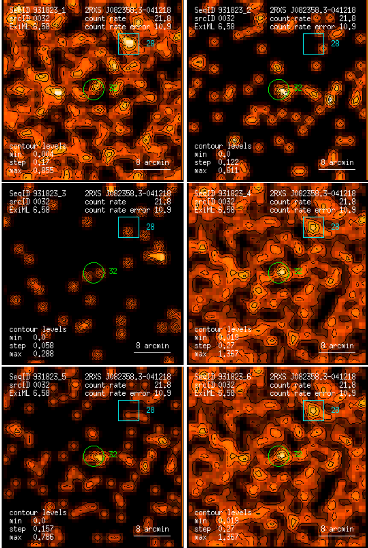
Figure 32: RASS 931823: detection 0032: band rate images, Gaussian filter: (1) PSPC channels 11 – 41, (2) 52 – 90, (3) 91 – 201, (4) 11 – 235, (5) 52 – 201, (6) 11 – 201. Broad band rates in counts/ks. Band rate contour levels in counts/ks/arcmin 2 .
