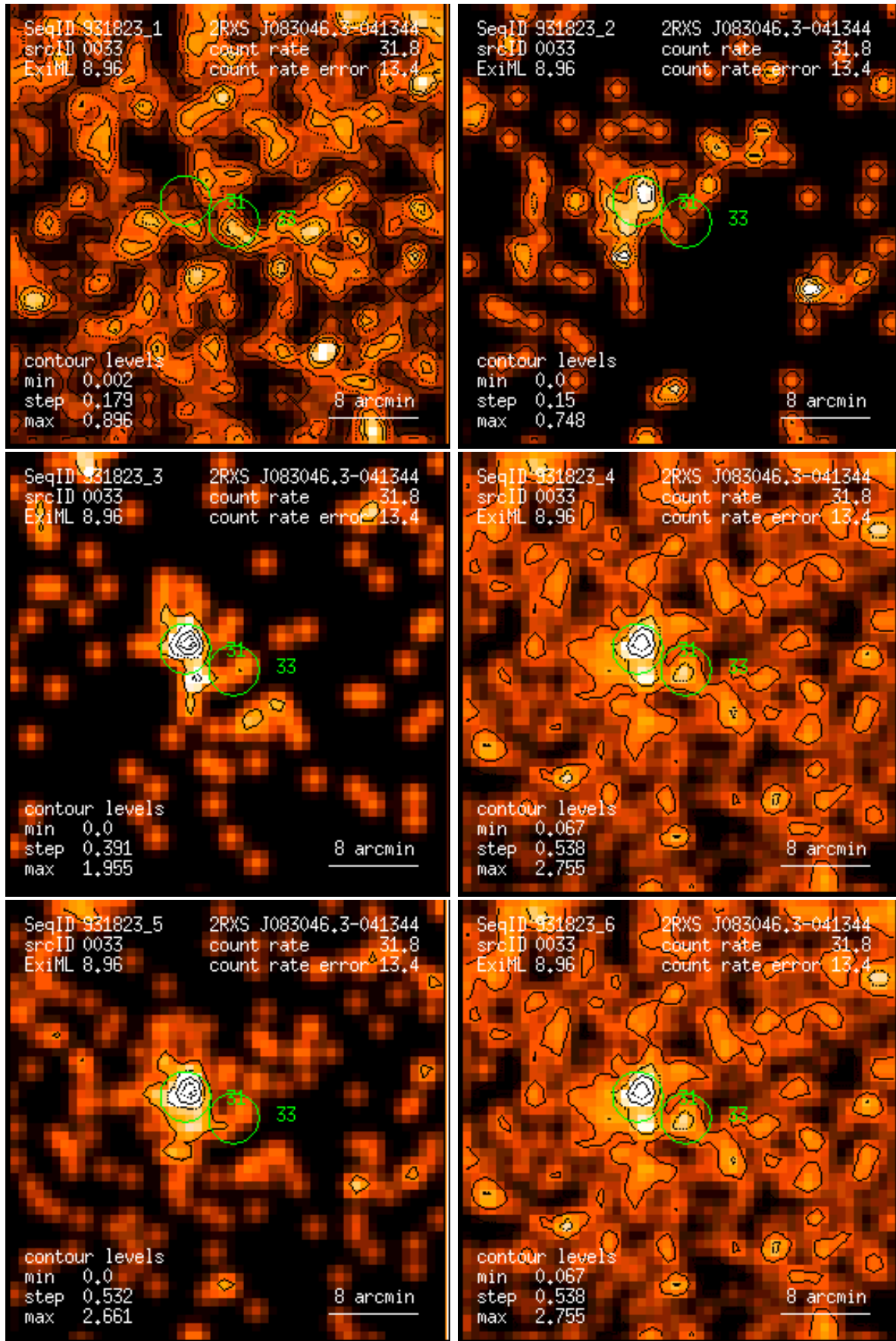
Figure 33: RASS 931823: detection 0033: band rate images, Gaussian filter: (1) PSPC channels 11 – 41, (2) 52 – 90, (3) 91 – 201, (4) 11 – 235, (5) 52 – 201, (6) 11 – 201. Broad band rates in counts/ks. Band rate contour levels in counts/ks/arcmin 2 .
