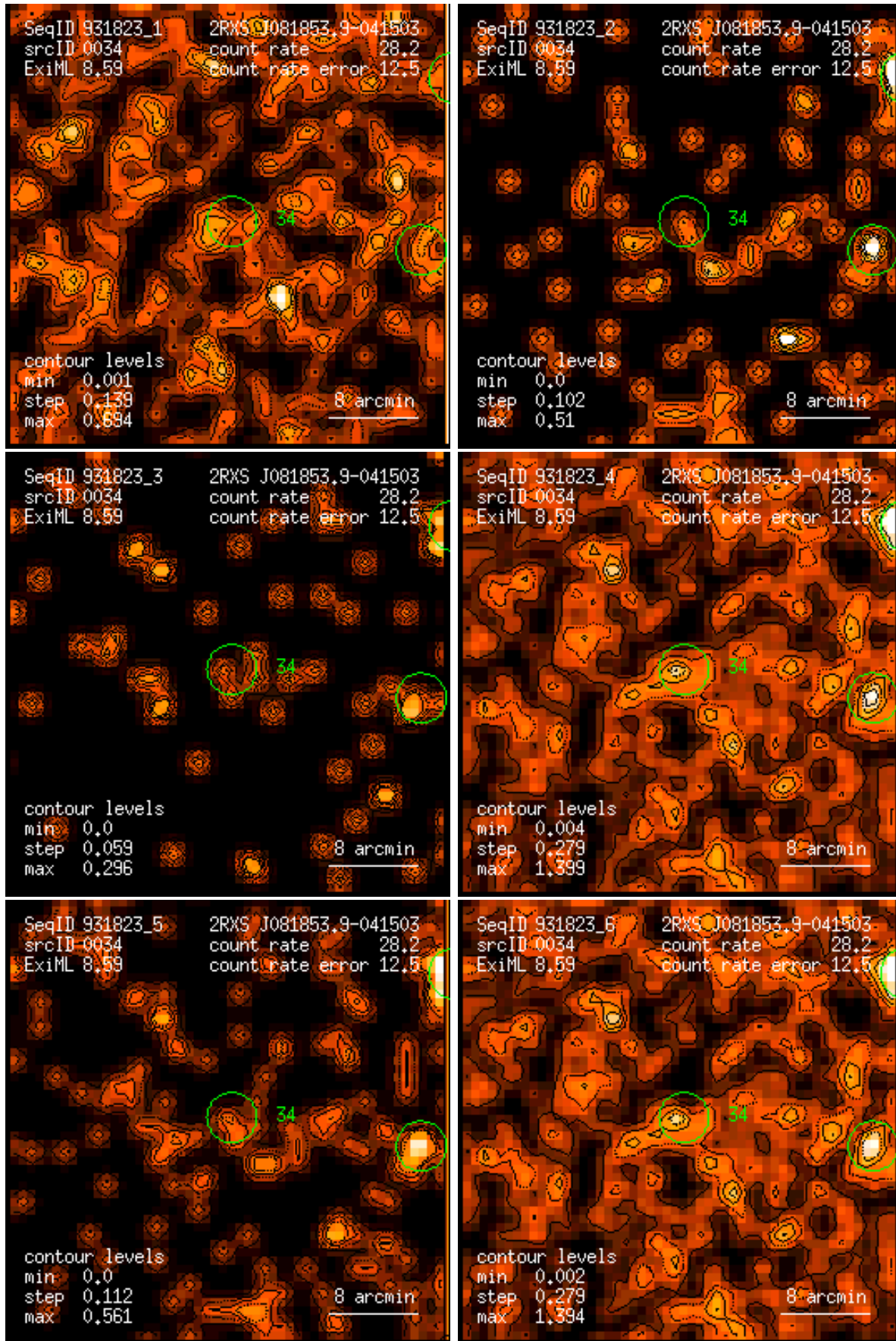
Figure 34: RASS 931823: detection 0034: band rate images, Gaussian filter: (1) PSPC channels 11 – 41, (2) 52 – 90, (3) 91 – 201, (4) 11 – 235, (5) 52 – 201, (6) 11 – 201. Broad band rates in counts/ks. Band rate contour levels in counts/ks/arcmin 2 .
