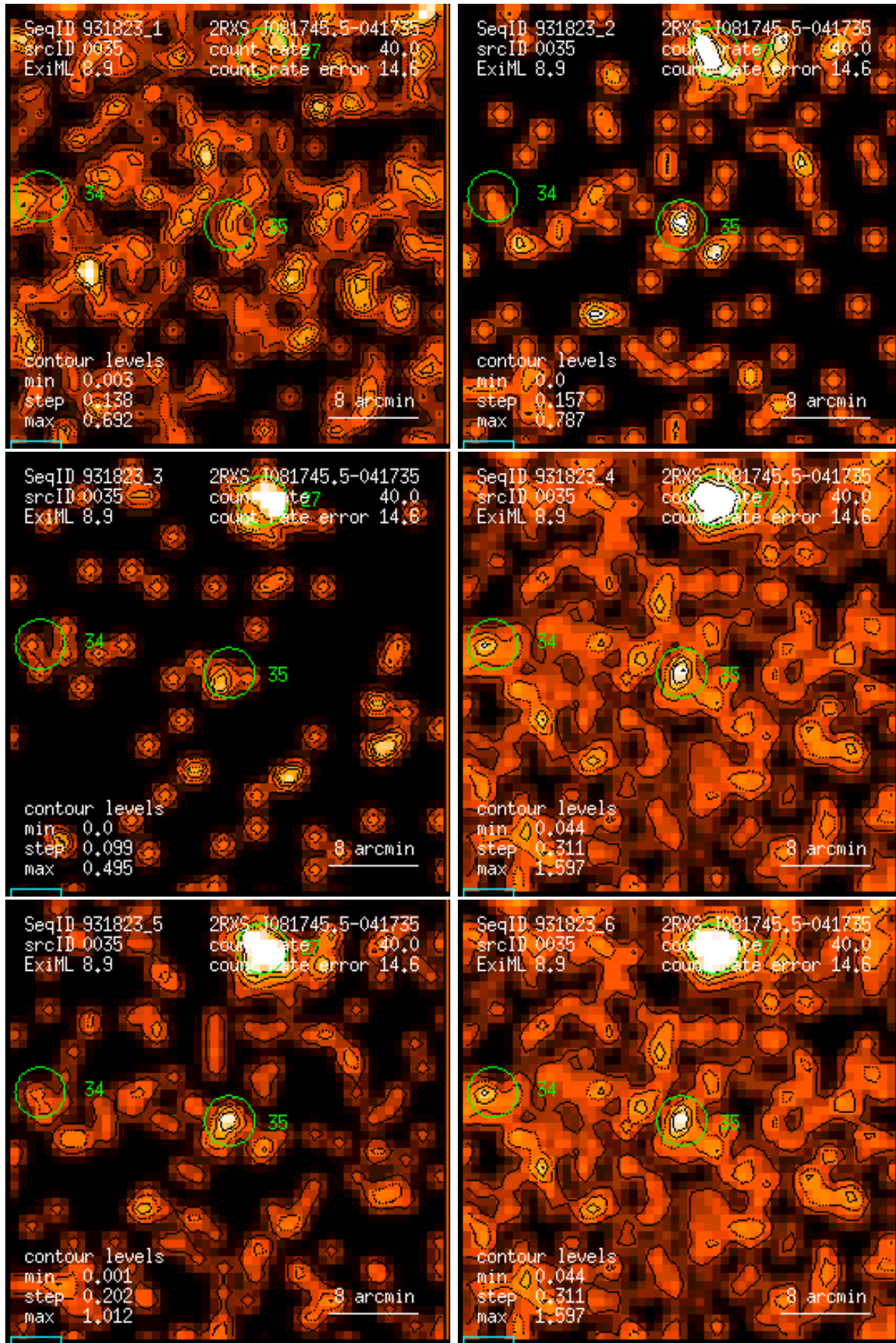
Figure 35: RASS 931823: detection 0035: band rate images, Gaussian filter: (1) PSPC channels 11 – 41, (2) 52 – 90, (3) 91 – 201, (4) 11 – 235, (5) 52 – 201, (6) 11 – 201. Broad band rates in counts/ks. Band rate contour levels in counts/ks/arcmin 2 .
