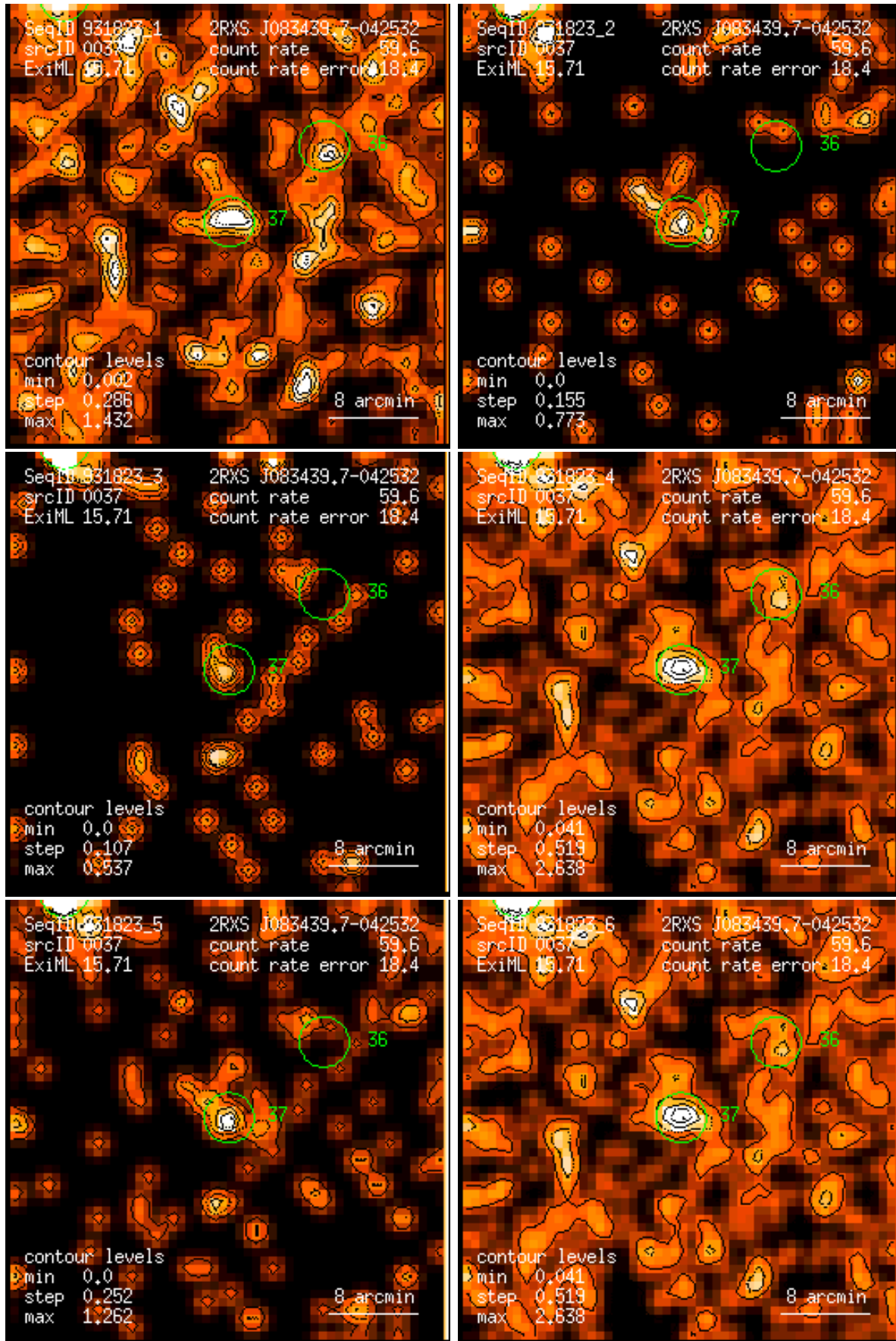
Figure 37: RASS 931823: detection 0037: band rate images, Gaussian filter: (1) PSPC channels 11 – 41, (2) 52 – 90, (3) 91 – 201, (4) 11 – 235, (5) 52 – 201, (6) 11 – 201. Broad band rates in counts/ks. Band rate contour levels in counts/ks/arcmin 2 .
