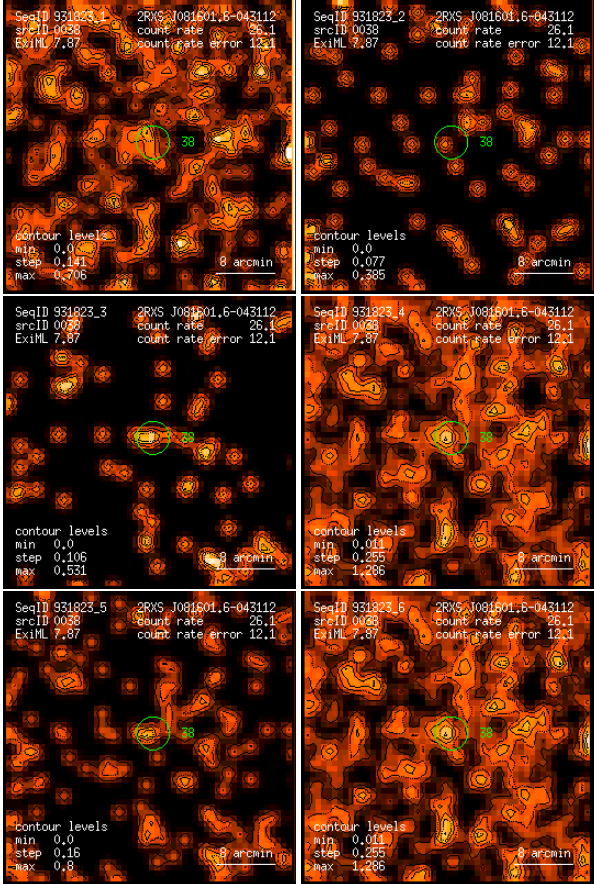
Figure 38: RASS 931823: detection 0038: band rate images, Gaussian filter: (1) PSPC channels 11 – 41, (2) 52 – 90, (3) 91 – 201, (4) 11 – 235, (5) 52 – 201, (6) 11 – 201. Broad band rates in counts/ks. Band rate contour levels in counts/ks/arcmin 2 .
