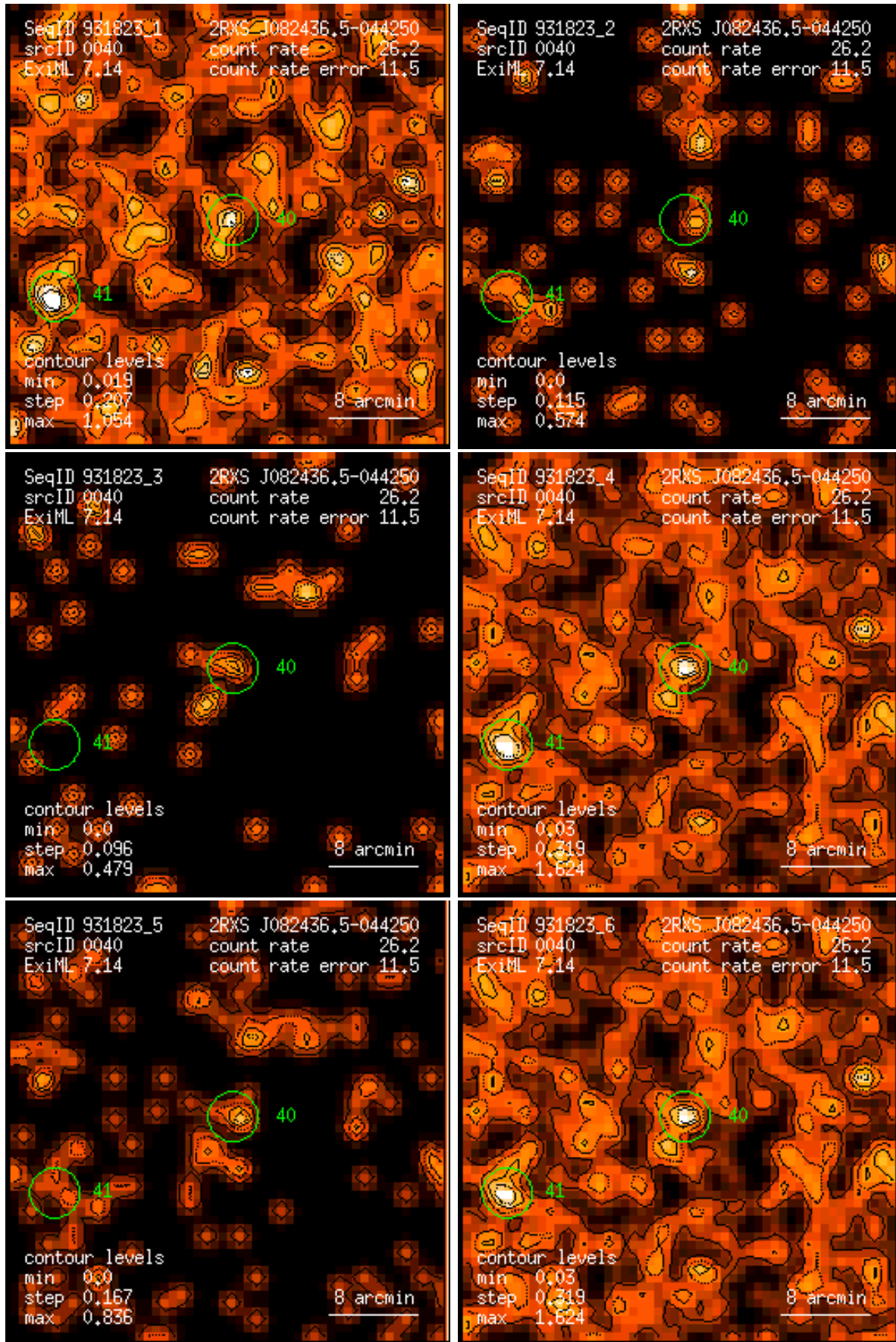
Figure 40: RASS 931823: detection 0040: band rate images, Gaussian filter: (1) PSPC channels 11 – 41, (2) 52 – 90, (3) 91 – 201, (4) 11 – 235, (5) 52 – 201, (6) 11 – 201. Broad band rates in counts/ks. Band rate contour levels in counts/ks/arcmin 2 .
