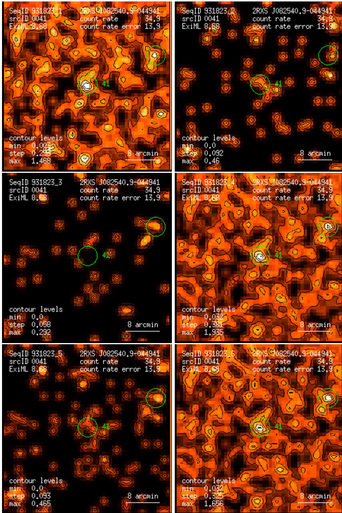
Figure 41: RASS 931823: detection 0041: band rate images, Gaussian filter: (1) PSPC channels 11 – 41, (2) 52 – 90, (3) 91 – 201, (4) 11 – 235, (5) 52 – 201, (6) 11 – 201. Broad band rates in counts/ks. Band rate contour levels in counts/ks/arcmin 2 .
