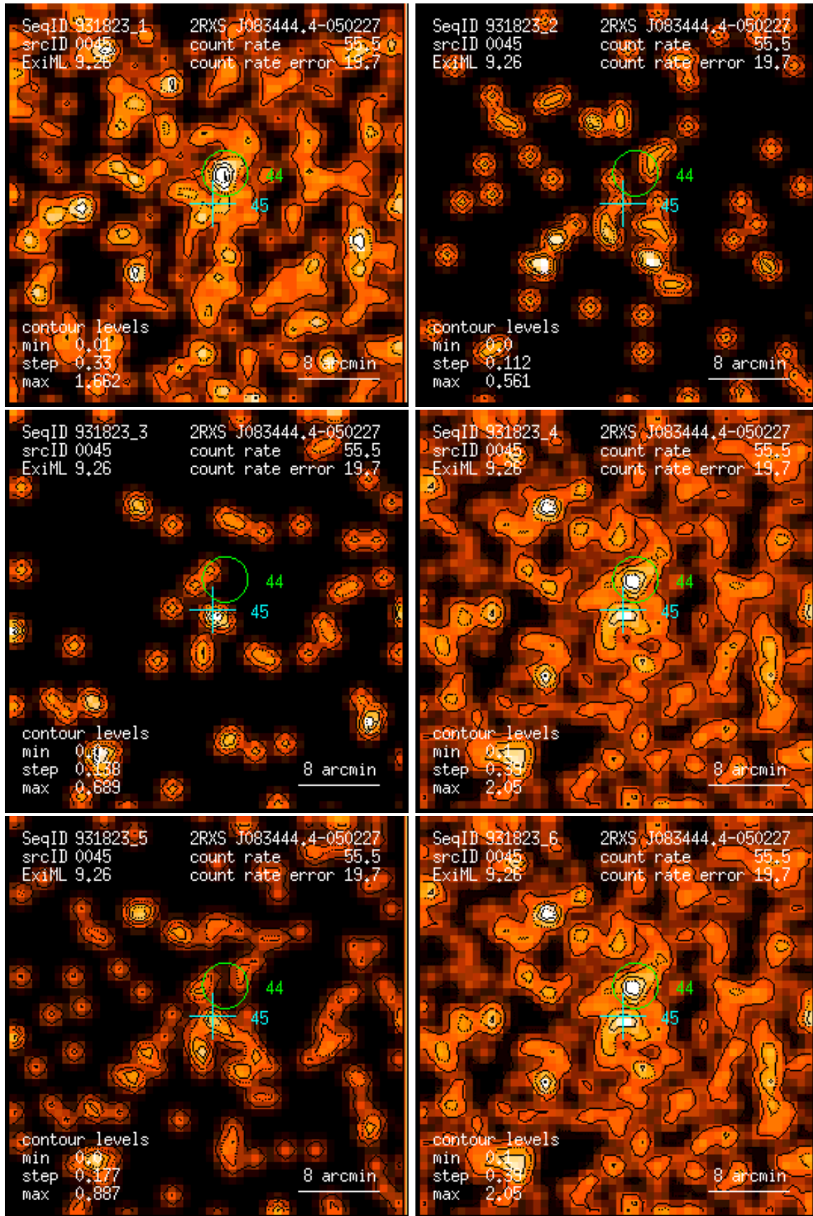
Figure 45: RASS 931823: detection 0045: band rate images, Gaussian filter: (1) PSPC channels 11 – 41, (2) 52 – 90, (3) 91 – 201, (4) 11 – 235, (5) 52 – 201, (6) 11 – 201. Broad band rates in counts/ks. Band rate contour levels in counts/ks/arcmin 2 .
