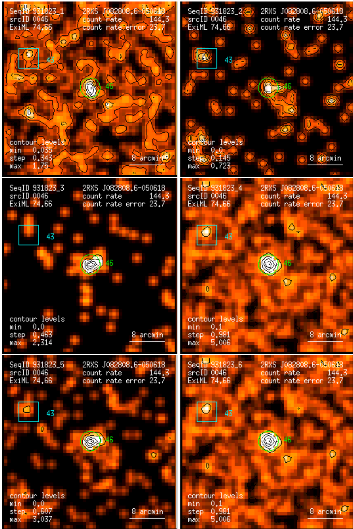
Figure 46: RASS 931823: detection 0046: band rate images, Gaussian filter: (1) PSPC channels 11 – 41, (2) 52 – 90, (3) 91 – 201, (4) 11 – 235, (5) 52 – 201, (6) 11 – 201. Broad band rates in counts/ks. Band rate contour levels in counts/ks/arcmin 2 .
