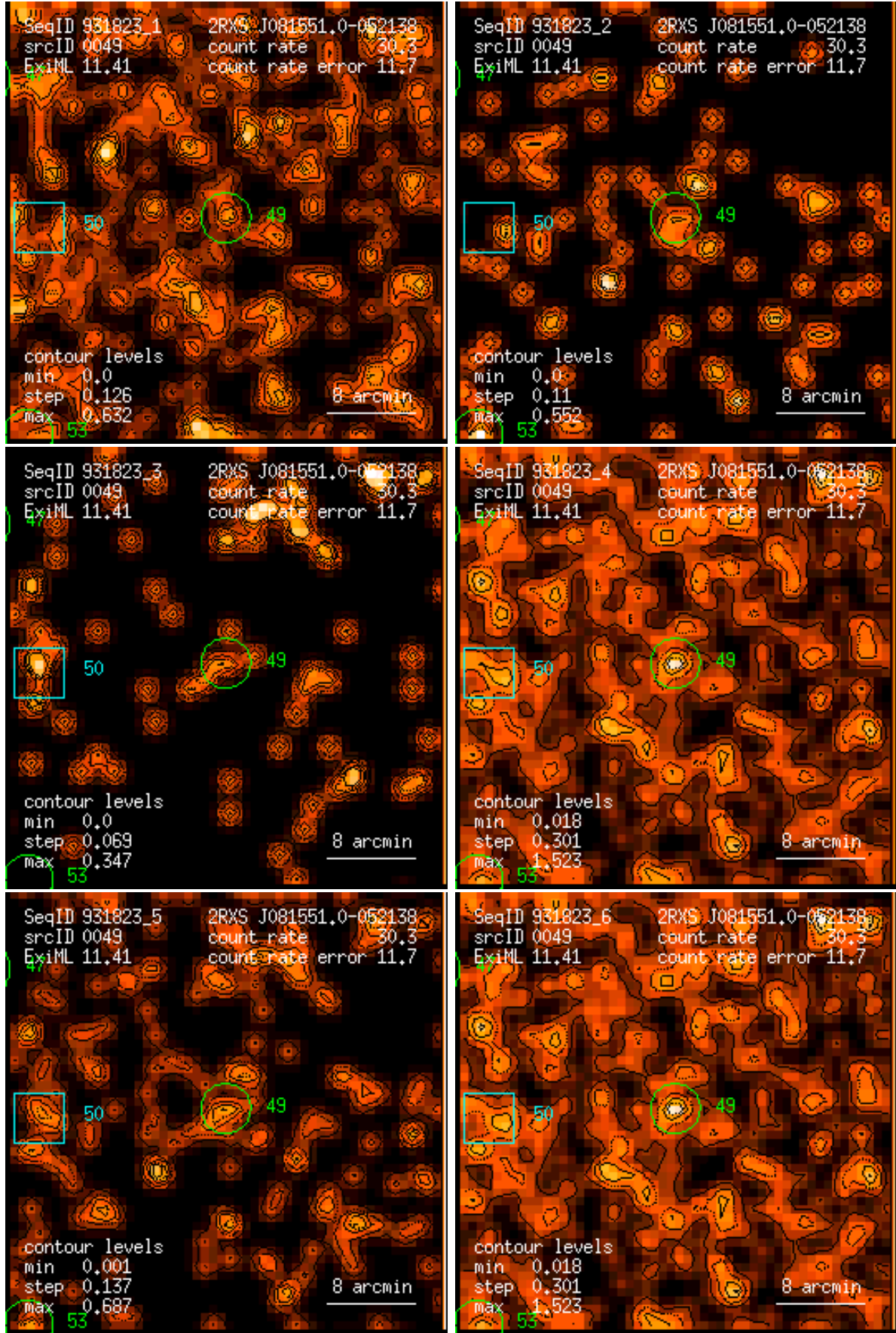
Figure 49: RASS 931823: detection 0049: band rate images, Gaussian filter: (1) PSPC channels 11 – 41, (2) 52 – 90, (3) 91 – 201, (4) 11 – 235, (5) 52 – 201, (6) 11 – 201. Broad band rates in counts/ks. Band rate contour levels in counts/ks/arcmin 2 .
