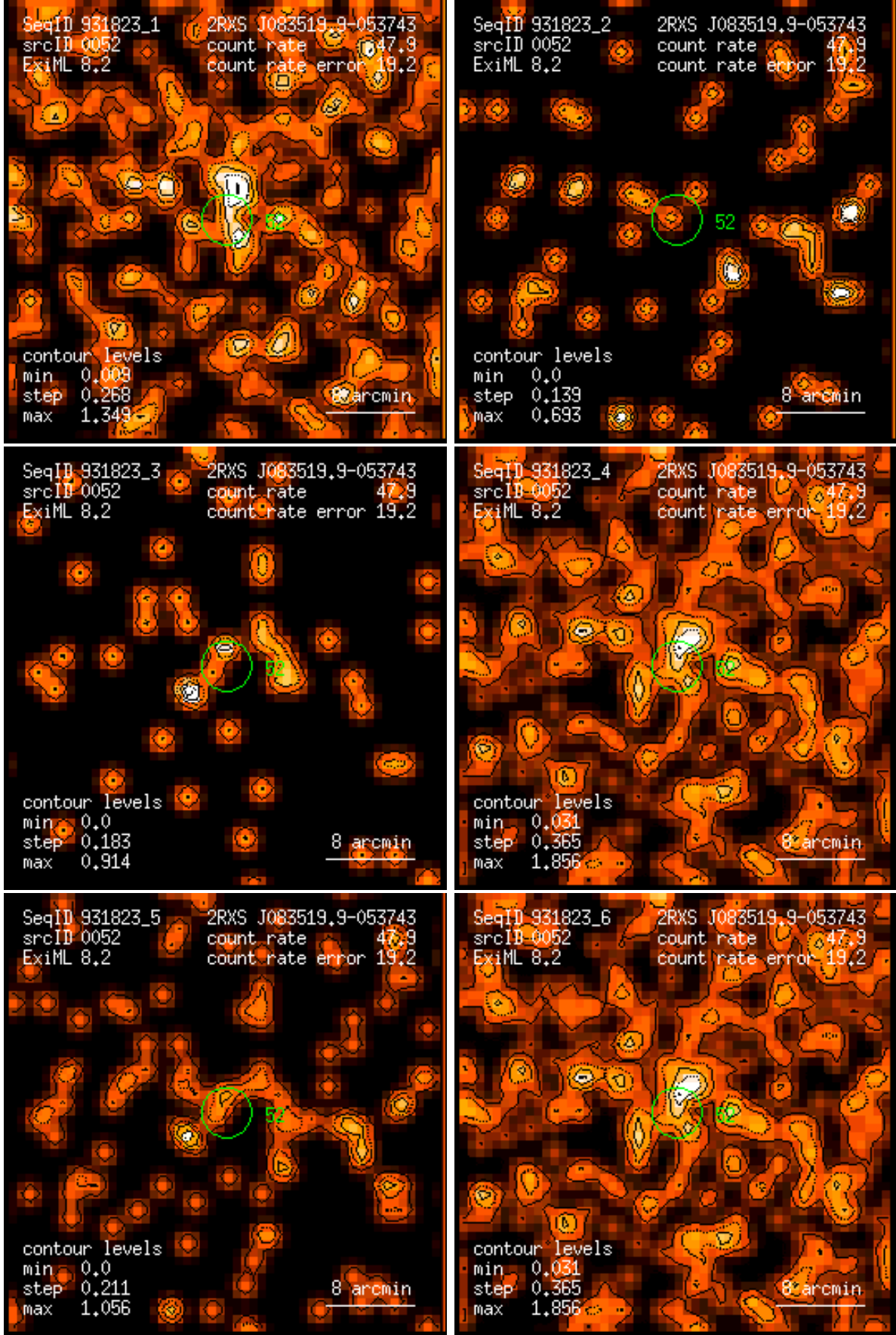
Figure 52: RASS 931823: detection 0052: band rate images, Gaussian filter: (1) PSPC channels 11 – 41, (2) 52 – 90, (3) 91 – 201, (4) 11 – 235, (5) 52 – 201, (6) 11 – 201. Broad band rates in counts/ks. Band rate contour levels in counts/ks/arcmin 2 .
