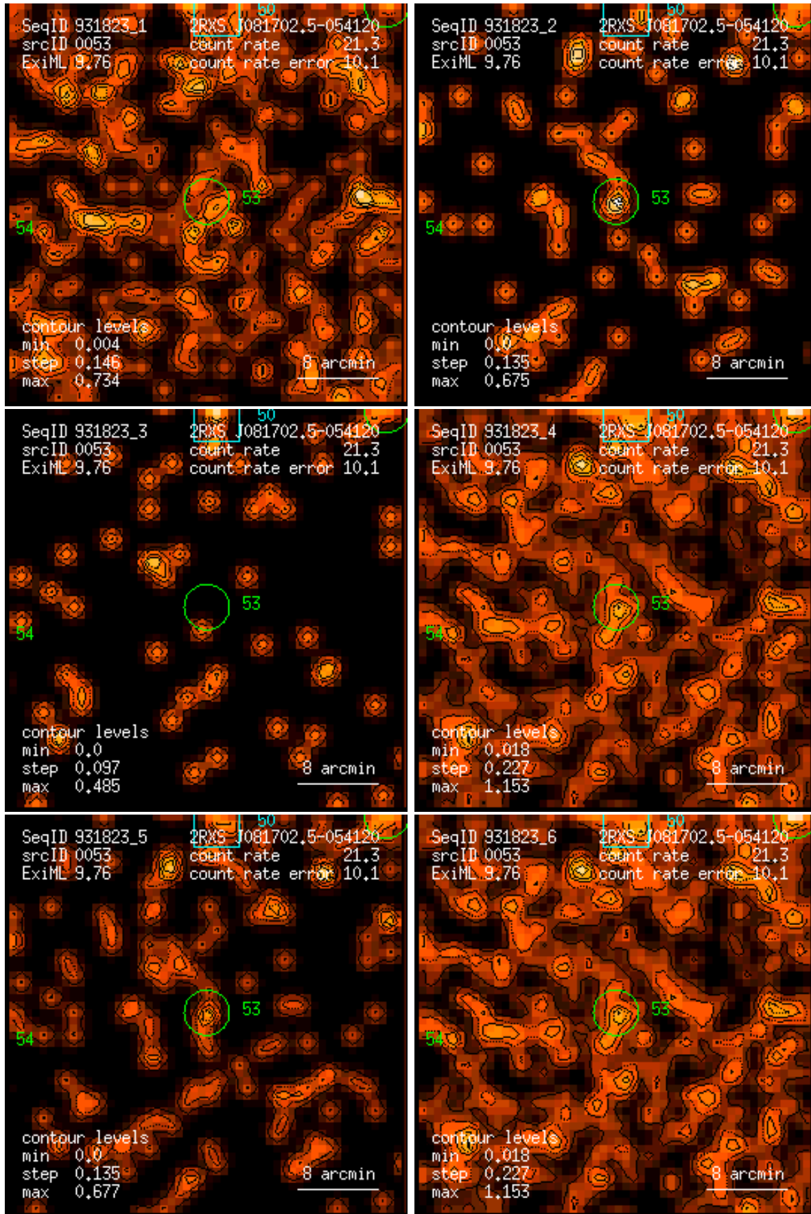
Figure 53: RASS 931823: detection 0053: band rate images, Gaussian filter: (1) PSPC channels 11 – 41, (2) 52 – 90, (3) 91 – 201, (4) 11 – 235, (5) 52 – 201, (6) 11 – 201. Broad band rates in counts/ks. Band rate contour levels in counts/ks/arcmin 2 .
