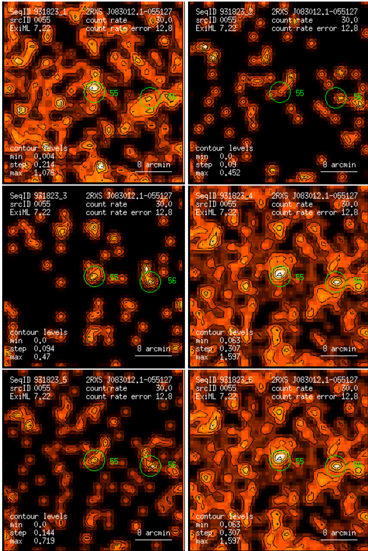
Figure 55: RASS 931823: detection 0055: band rate images, Gaussian filter: (1) PSPC channels 11 – 41, (2) 52 – 90, (3) 91 – 201, (4) 11 – 235, (5) 52 – 201, (6) 11 – 201. Broad band rates in counts/ks. Band rate contour levels in counts/ks/arcmin 2 .
