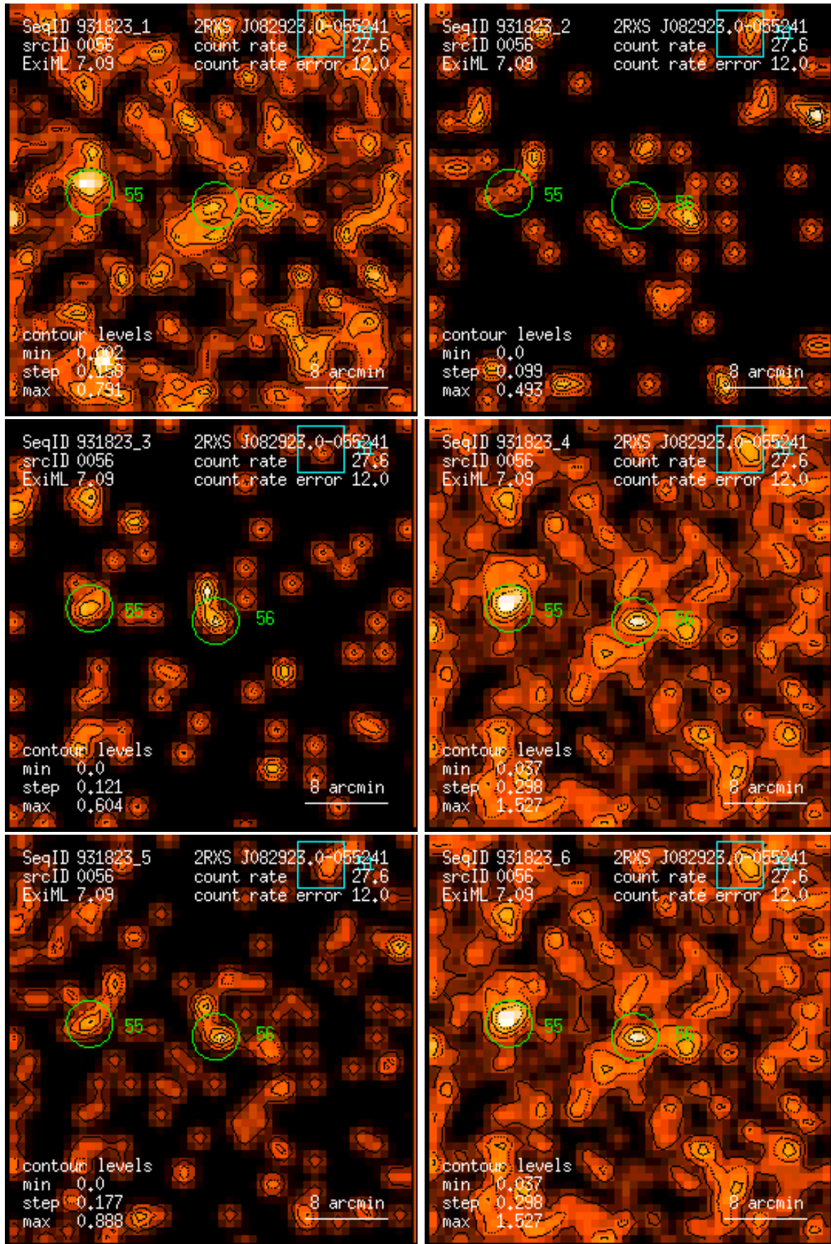
Figure 56: RASS 931823: detection 0056: band rate images, Gaussian filter: (1) PSPC channels 11 – 41, (2) 52 – 90, (3) 91 – 201, (4) 11 – 235, (5) 52 – 201, (6) 11 – 201. Broad band rates in counts/ks. Band rate contour levels in counts/ks/arcmin 2 .
