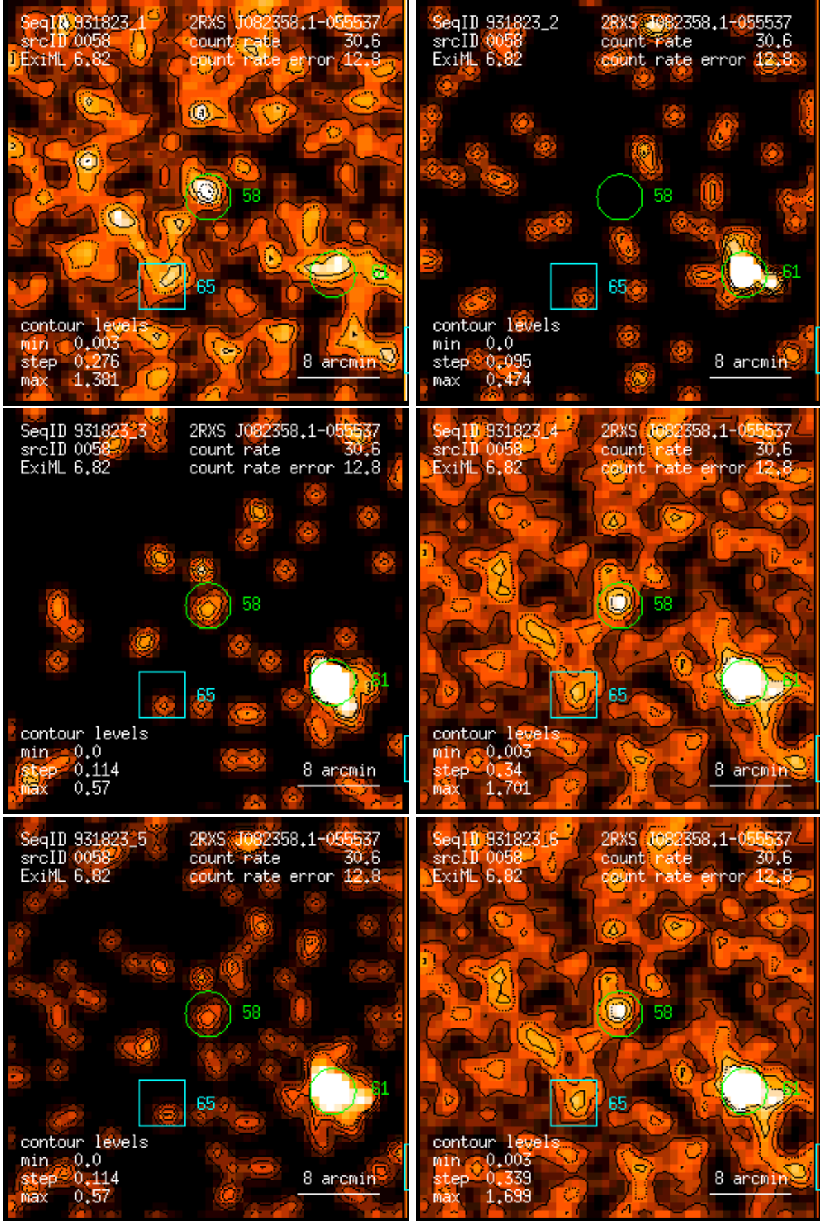
Figure 58: RASS 931823: detection 0058: band rate images, Gaussian filter: (1) PSPC channels 11 – 41, (2) 52 – 90, (3) 91 – 201, (4) 11 – 235, (5) 52 – 201, (6) 11 – 201. Broad band rates in counts/ks. Band rate contour levels in counts/ks/arcmin 2 .
