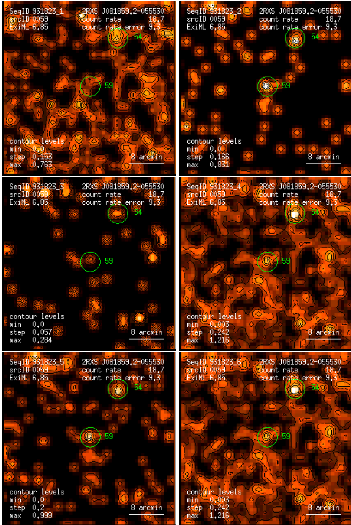
Figure 59: RASS 931823: detection 0059: band rate images, Gaussian filter: (1) PSPC channels 11 – 41, (2) 52 – 90, (3) 91 – 201, (4) 11 – 235, (5) 52 – 201, (6) 11 – 201. Broad band rates in counts/ks. Band rate contour levels in counts/ks/arcmin 2 .
