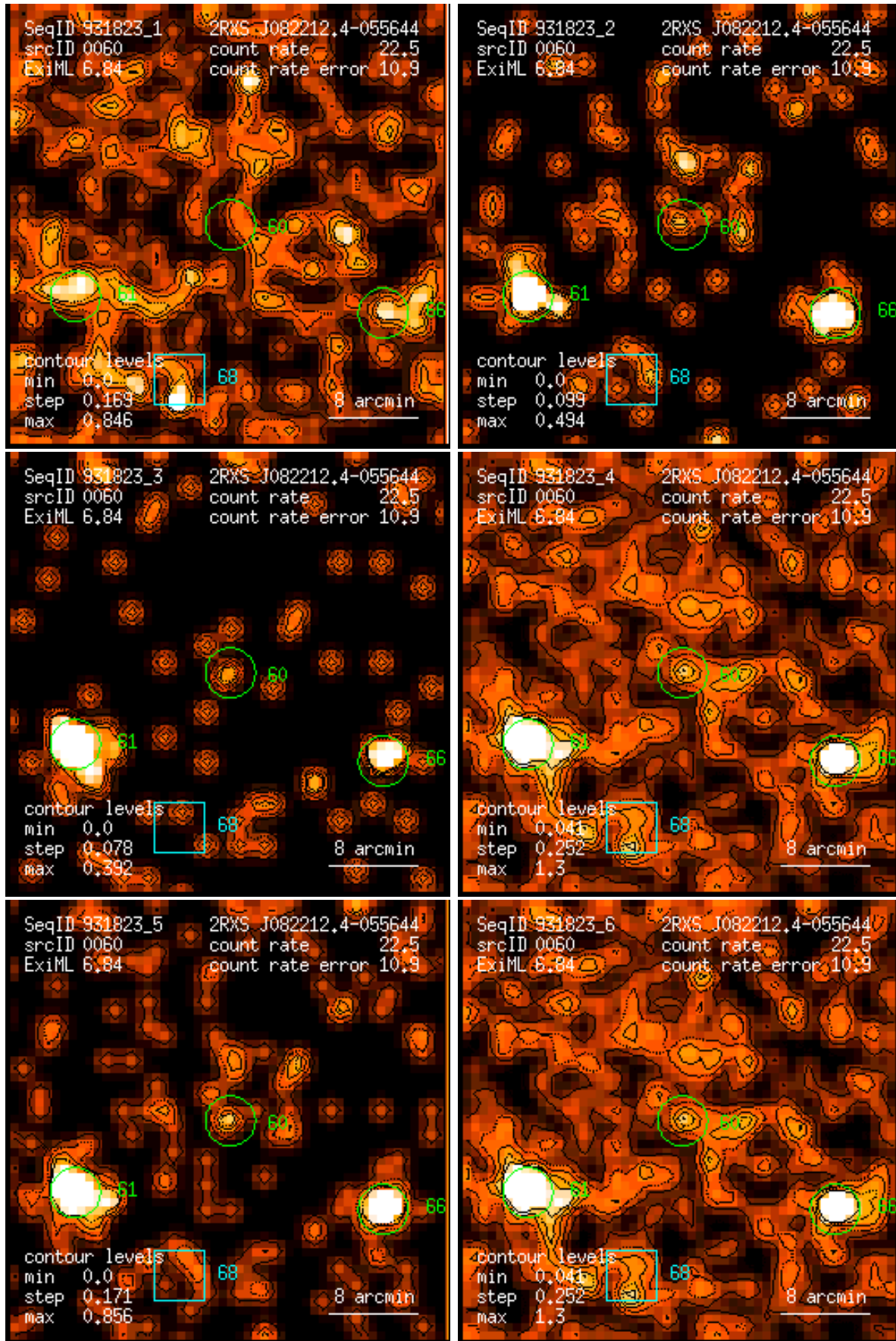
Figure 60: RASS 931823: detection 0060: band rate images, Gaussian filter: (1) PSPC channels 11 – 41, (2) 52 – 90, (3) 91 – 201, (4) 11 – 235, (5) 52 – 201, (6) 11 – 201. Broad band rates in counts/ks. Band rate contour levels in counts/ks/arcmin 2 .
