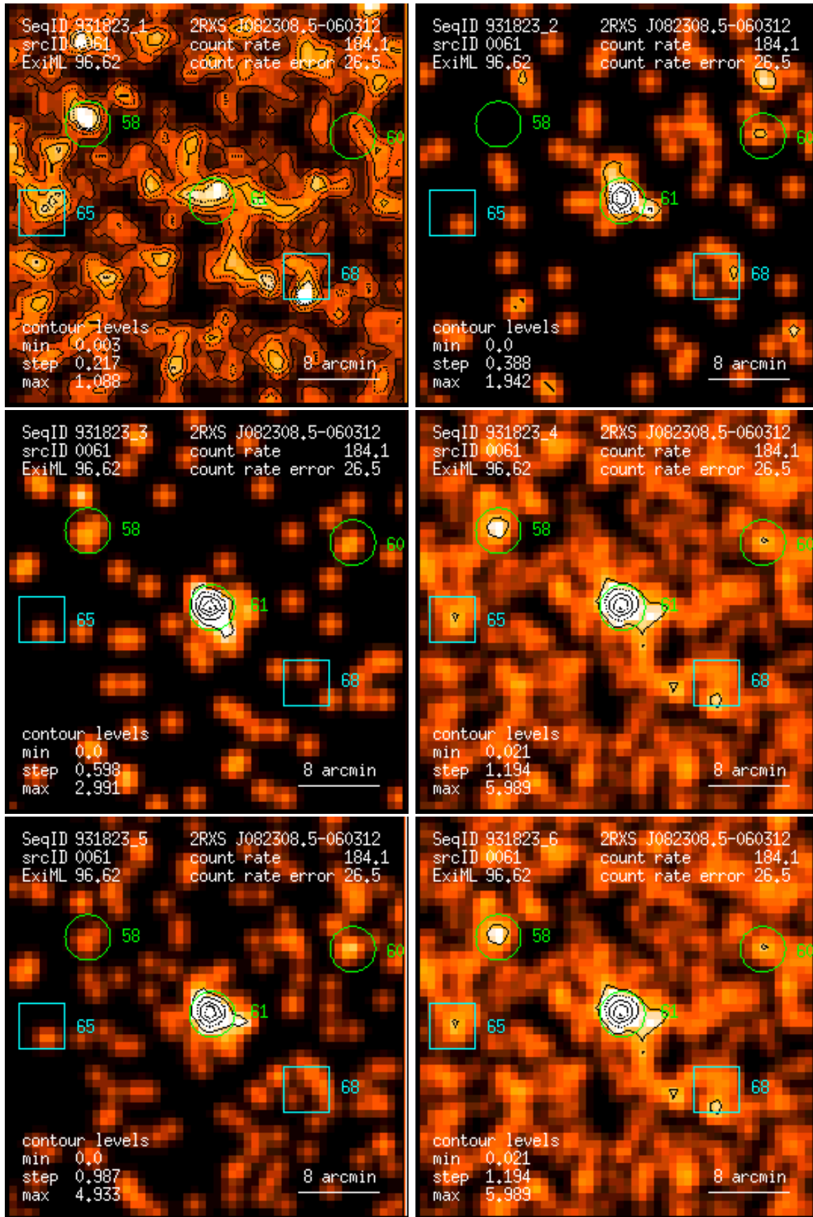
Figure 61: RASS 931823: detection 0061: band rate images, Gaussian filter: (1) PSPC channels 11 – 41, (2) 52 – 90, (3) 91 – 201, (4) 11 – 235, (5) 52 – 201, (6) 11 – 201. Broad band rates in counts/ks. Band rate contour levels in counts/ks/arcmin 2 .
