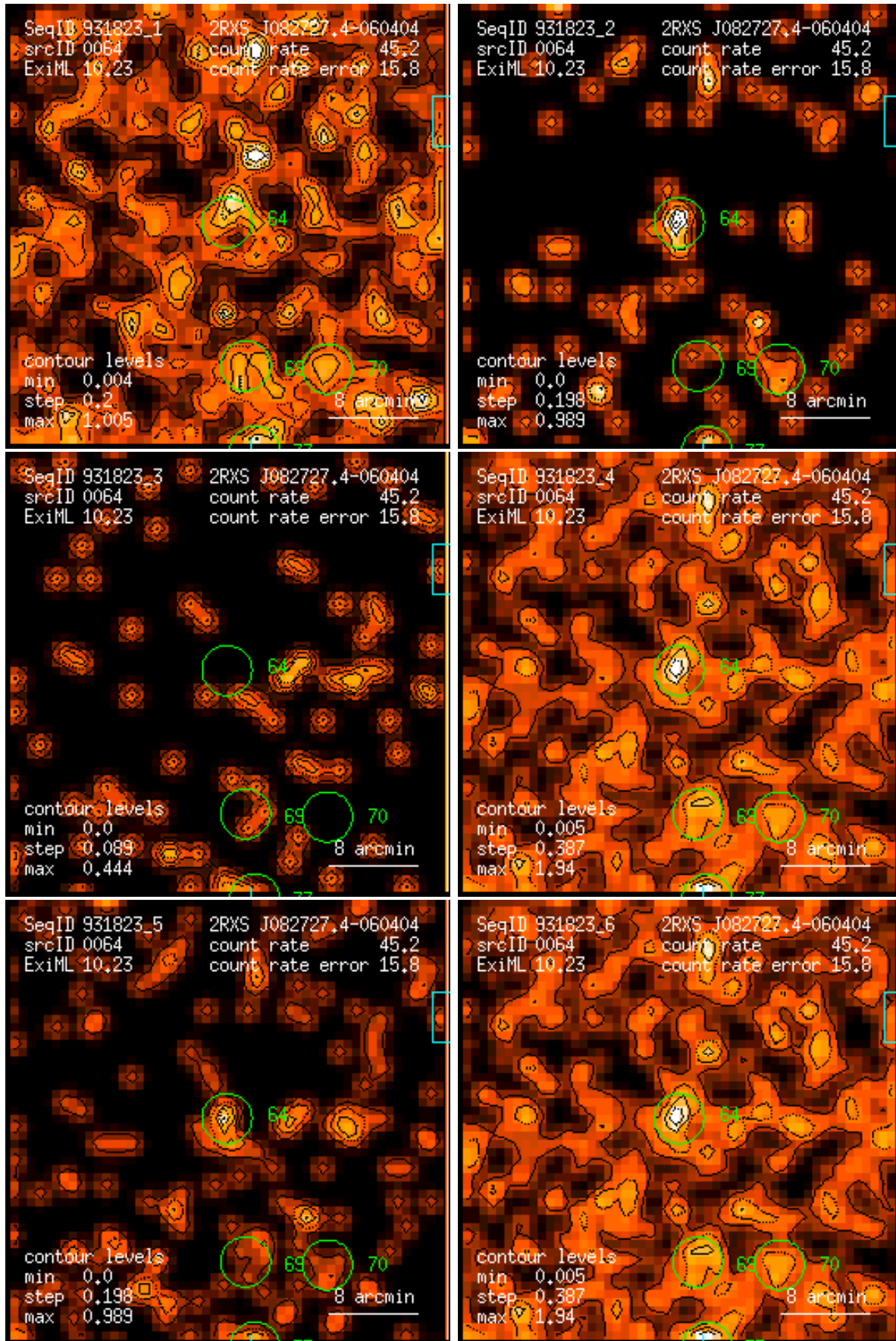
Figure 64: RASS 931823: detection 0064: band rate images, Gaussian filter: (1) PSPC channels 11 – 41, (2) 52 – 90, (3) 91 – 201, (4) 11 – 235, (5) 52 – 201, (6) 11 – 201. Broad band rates in counts/ks. Band rate contour levels in counts/ks/arcmin 2 .
