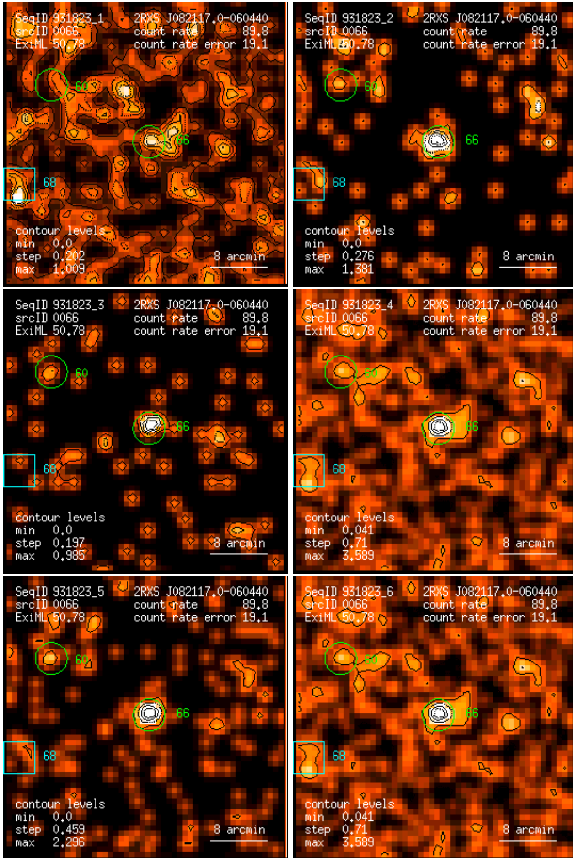
Figure 66: RASS 931823: detection 0066: band rate images, Gaussian filter: (1) PSPC channels 11 – 41, (2) 52 – 90, (3) 91 – 201, (4) 11 – 235, (5) 52 – 201, (6) 11 – 201. Broad band rates in counts/ks. Band rate contour levels in counts/ks/arcmin 2 .
