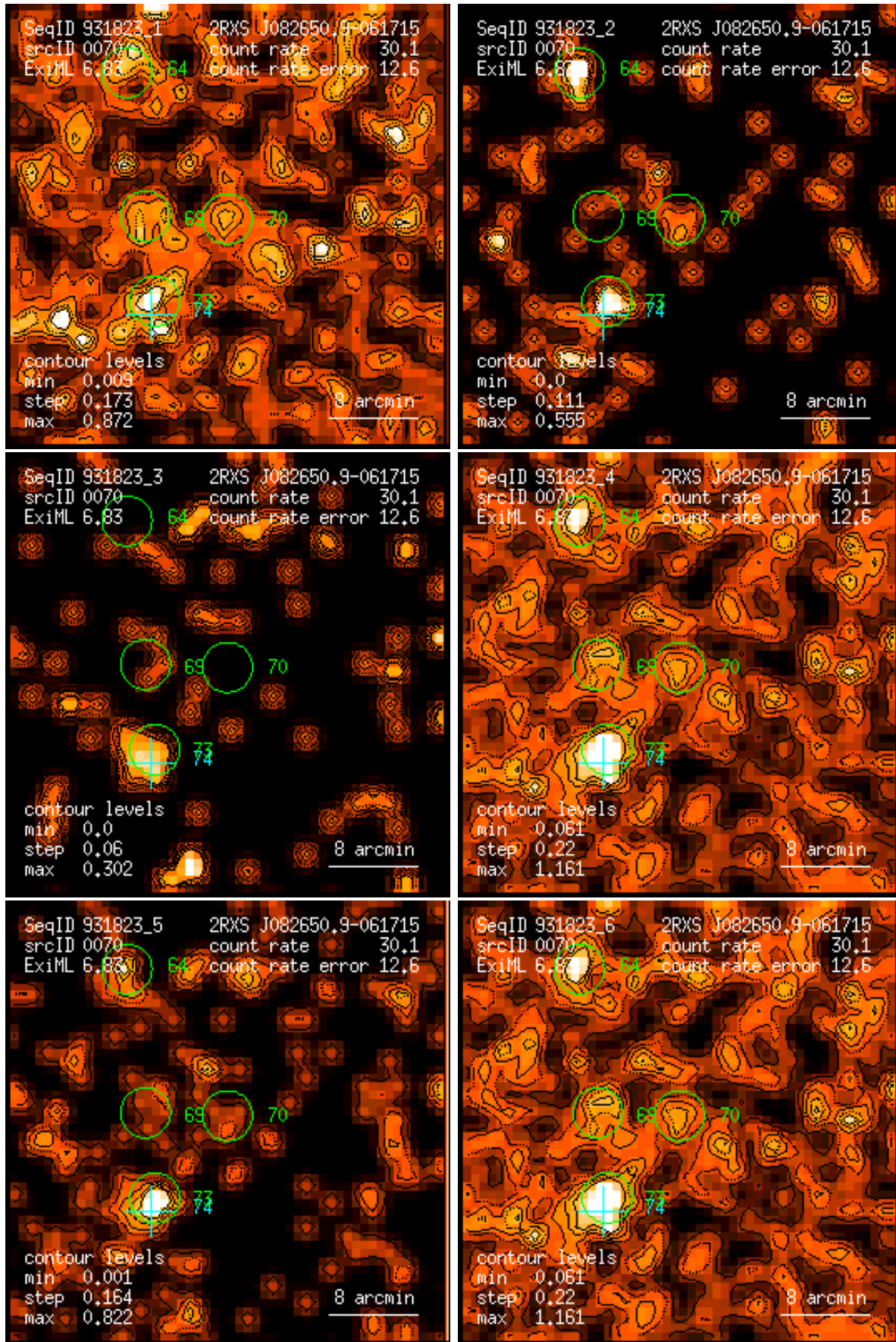
Figure 70: RASS 931823: detection 0070: band rate images, Gaussian filter: (1) PSPC channels 11 – 41, (2) 52 – 90, (3) 91 – 201, (4) 11 – 235, (5) 52 – 201, (6) 11 – 201. Broad band rates in counts/ks. Band rate contour levels in counts/ks/arcmin 2 .
