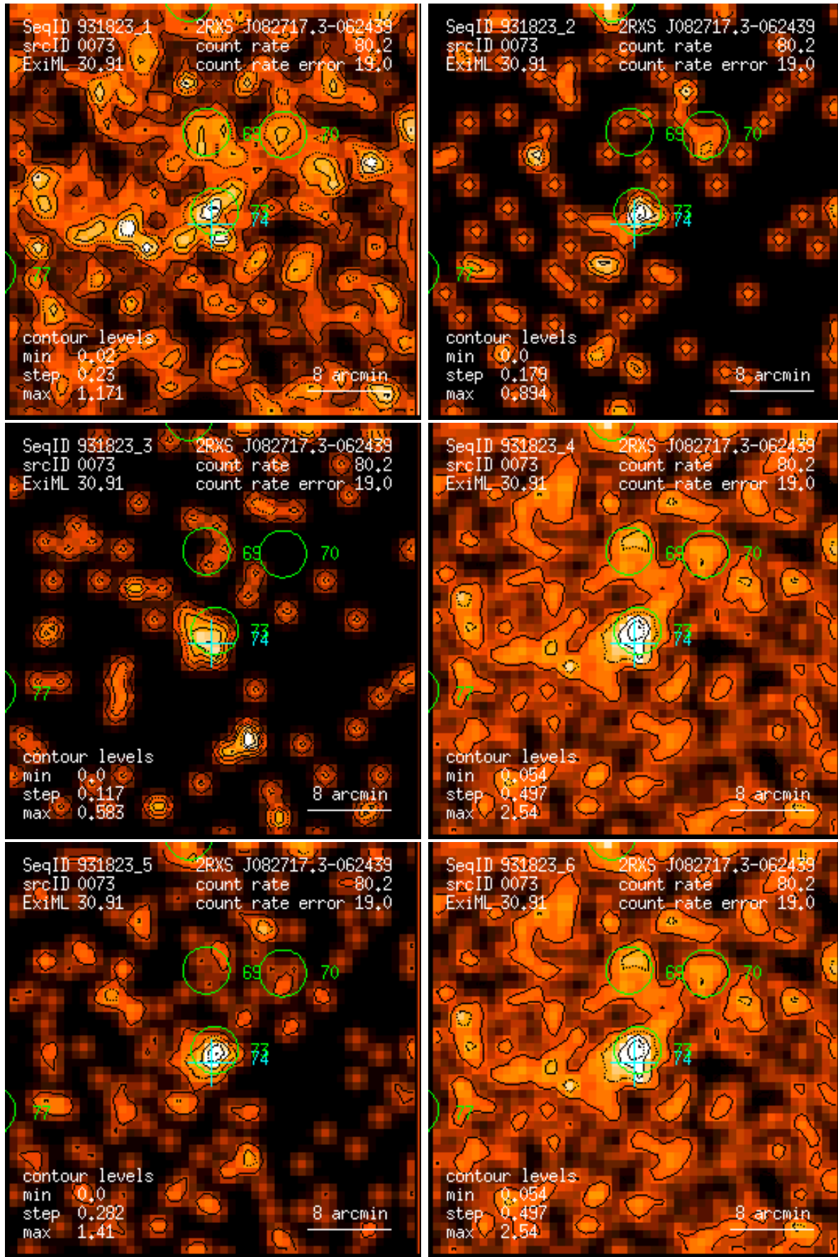
Figure 73: RASS 931823: detection 0073: band rate images, Gaussian filter: (1) PSPC channels 11 – 41, (2) 52 – 90, (3) 91 – 201, (4) 11 – 235, (5) 52 – 201, (6) 11 – 201. Broad band rates in counts/ks. Band rate contour levels in counts/ks/arcmin 2 .
